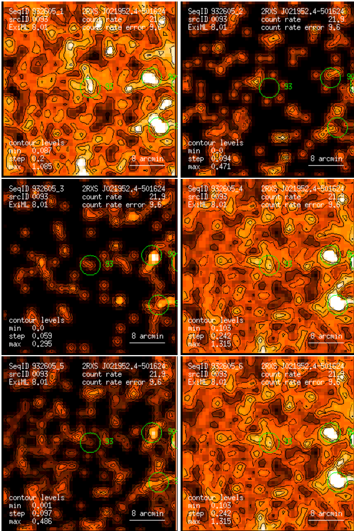
Figure 93: RASS 932605: detection 0093: band rate images, Gaussian filter: (1) PSPC channels 11 – 41, (2) 52 – 90, (3) 91 – 201, (4) 11 – 235, (5) 52 – 201, (6) 11 – 201. Broad band rates in counts/ks. Band rate contour levels in counts/ks/arcmin 2 .
