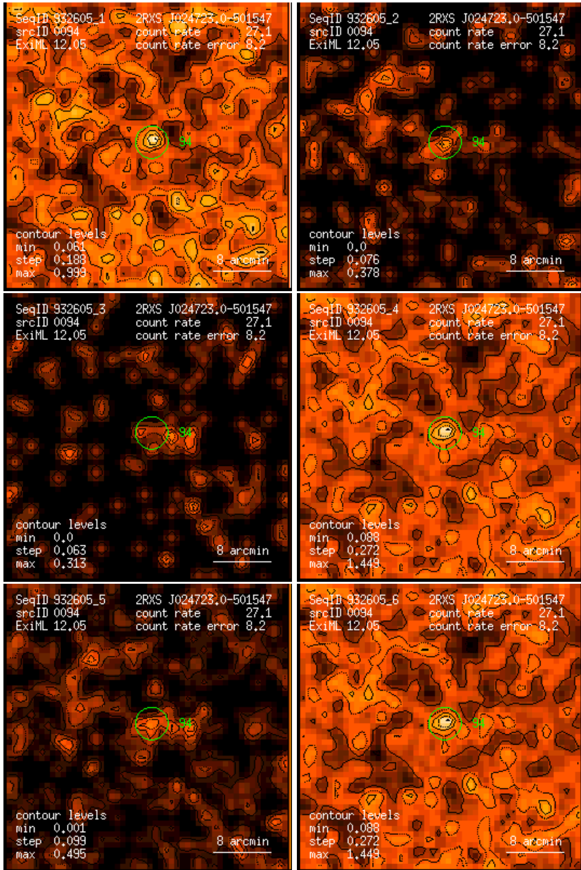
Figure 94: RASS 932605: detection 0094: band rate images, Gaussian filter: (1) PSPC channels 11 – 41, (2) 52 – 90, (3) 91 – 201, (4) 11 – 235, (5) 52 – 201, (6) 11 – 201. Broad band rates in counts/ks. Band rate contour levels in counts/ks/arcmin 2 .
