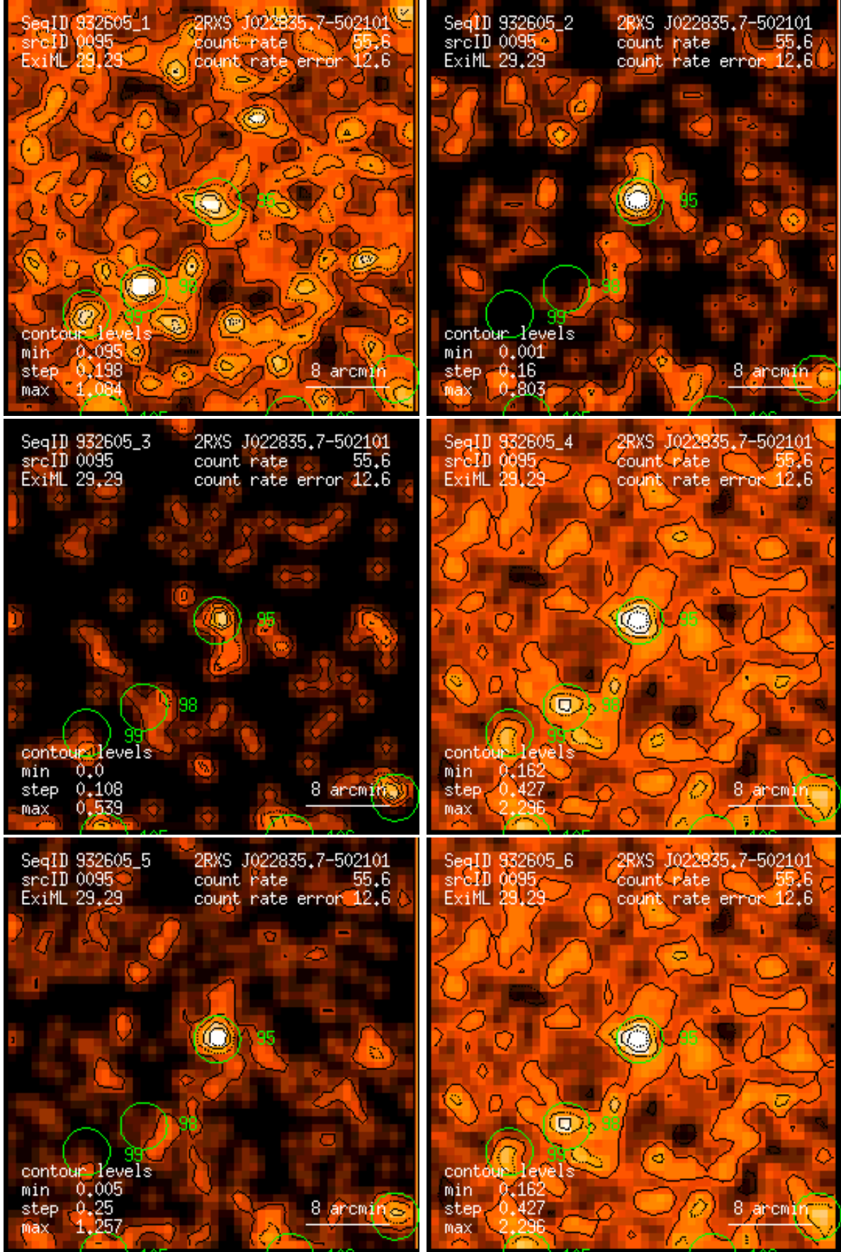
Figure 95: RASS 932605: detection 0095: band rate images, Gaussian filter: (1) PSPC channels 11 – 41, (2) 52 – 90, (3) 91 – 201, (4) 11 – 235, (5) 52 – 201, (6) 11 – 201. Broad band rates in counts/ks. Band rate contour levels in counts/ks/arcmin 2 .
