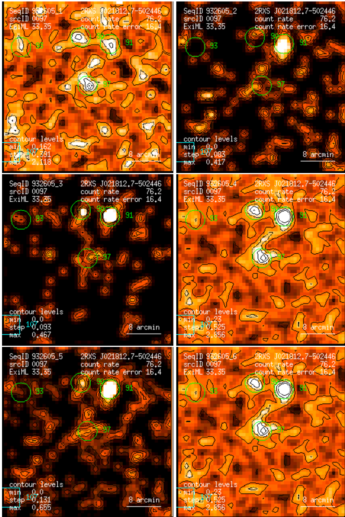
Figure 97: RASS 932605: detection 0097: band rate images, Gaussian filter: (1) PSPC channels 11 – 41, (2) 52 – 90, (3) 91 – 201, (4) 11 – 235, (5) 52 – 201, (6) 11 – 201. Broad band rates in counts/ks. Band rate contour levels in counts/ks/arcmin 2 .
