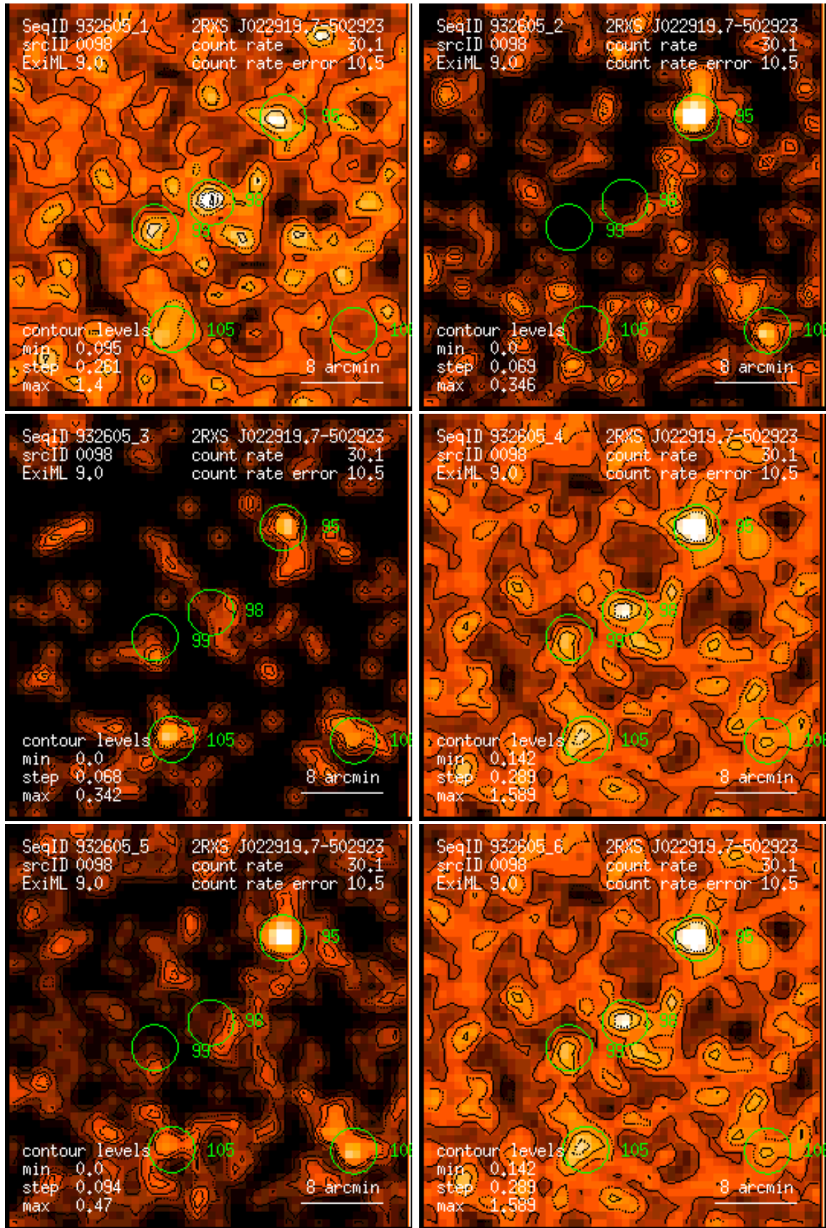
Figure 98: RASS 932605: detection 0098: band rate images, Gaussian filter: (1) PSPC channels 11 – 41, (2) 52 – 90, (3) 91 – 201, (4) 11 – 235, (5) 52 – 201, (6) 11 – 201. Broad band rates in counts/ks. Band rate contour levels in counts/ks/arcmin 2 .
