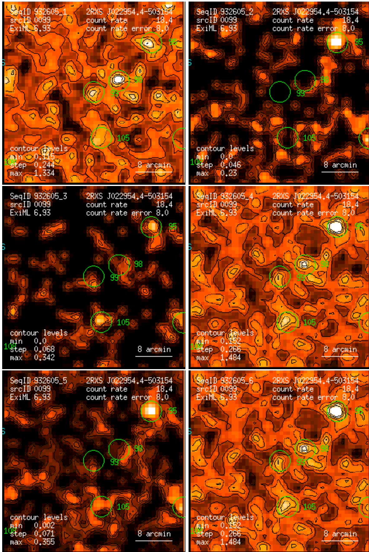
Figure 99: RASS 932605: detection 0099: band rate images, Gaussian filter: (1) PSPC channels 11 – 41, (2) 52 – 90, (3) 91 – 201, (4) 11 – 235, (5) 52 – 201, (6) 11 – 201. Broad band rates in counts/ks. Band rate contour levels in counts/ks/arcmin 2 .
