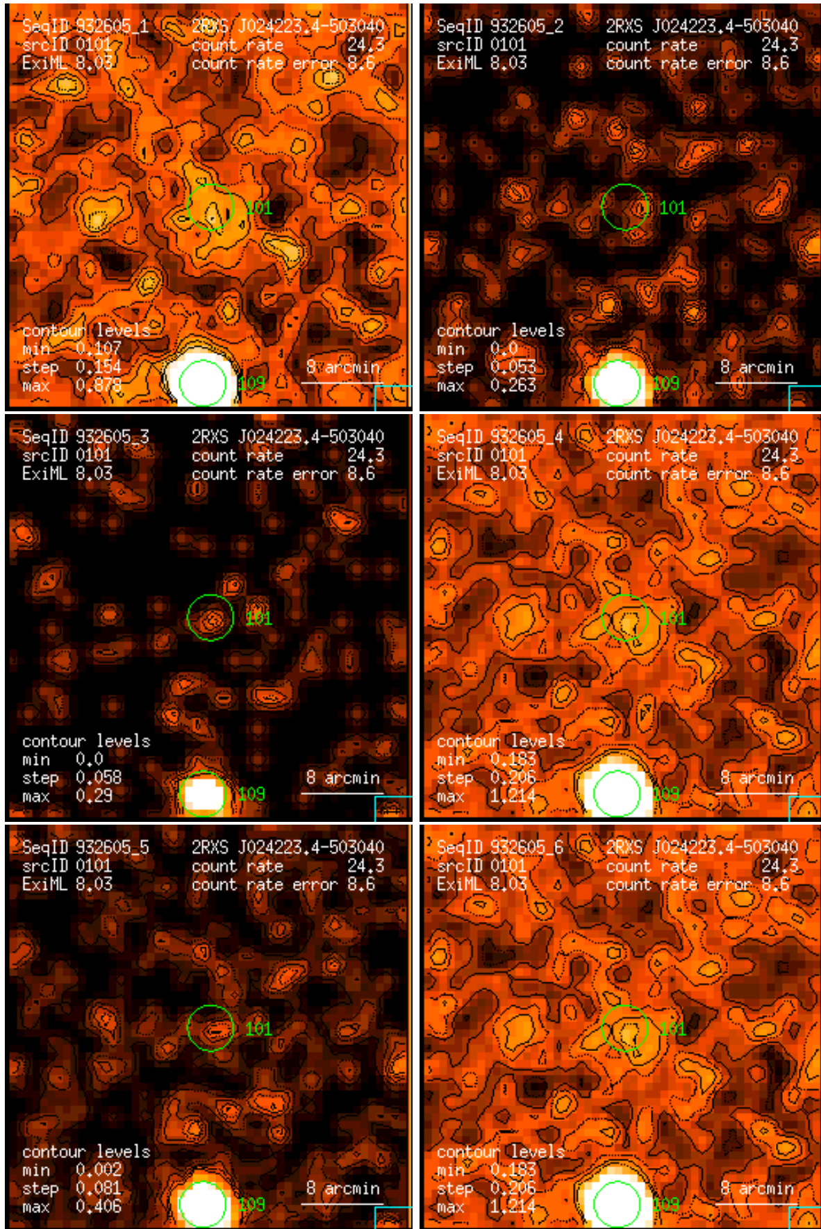
Figure 101: RASS 932605: detection 0101: band rate images, Gaussian filter: (1) PSPC channels 11 – 41, (2) 52 – 90, (3) 91 – 201, (4) 11 – 235, (5) 52 – 201, (6) 11 – 201. Broad band rates in counts/ks. Band rate contour levels in counts/ks/arcmin 2 .
