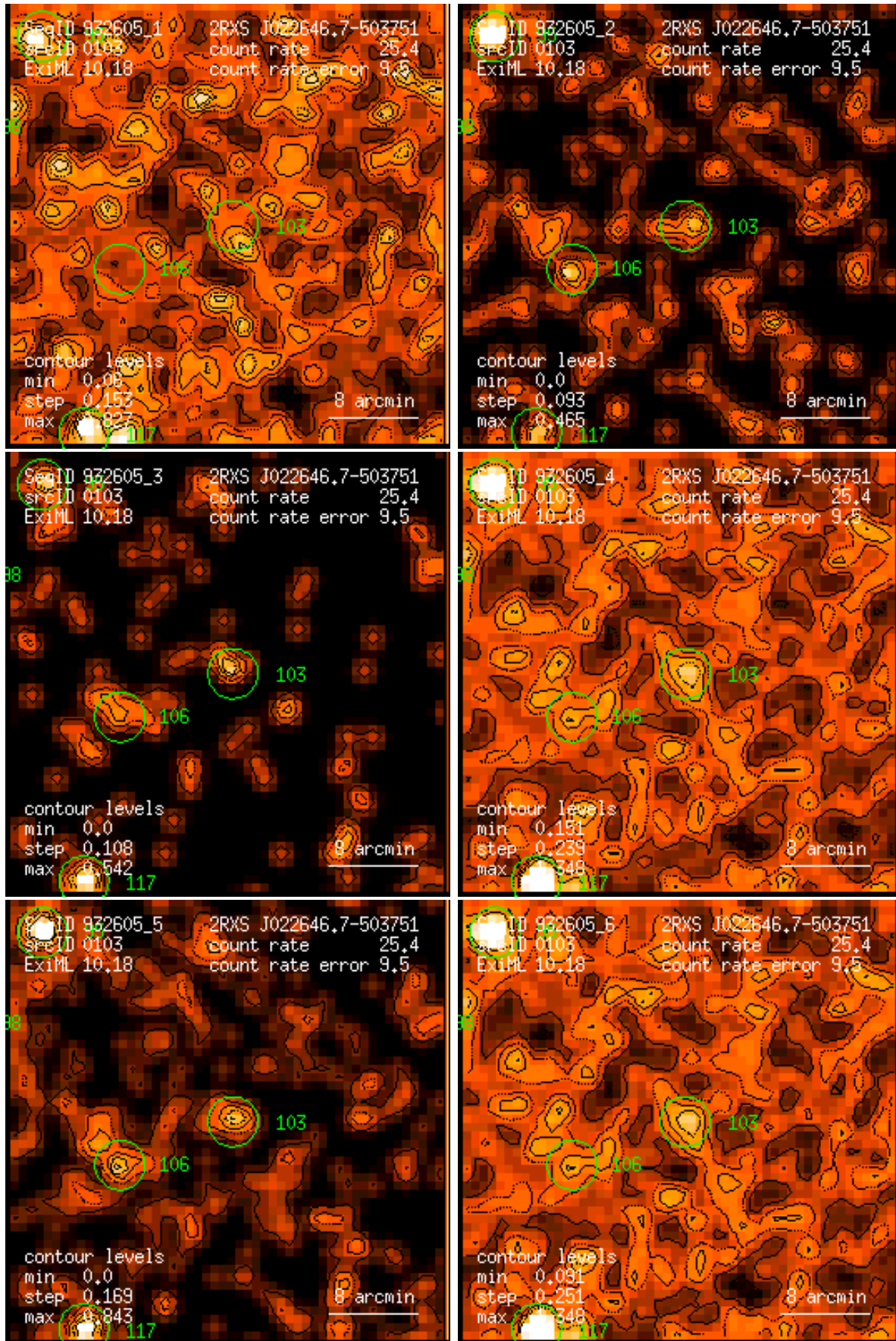
Figure 103: RASS 932605: detection 0103: band rate images, Gaussian filter: (1) PSPC channels 11 – 41, (2) 52 – 90, (3) 91 – 201, (4) 11 – 235, (5) 52 – 201, (6) 11 – 201. Broad band rates in counts/ks. Band rate contour levels in counts/ks/arcmin 2 .
