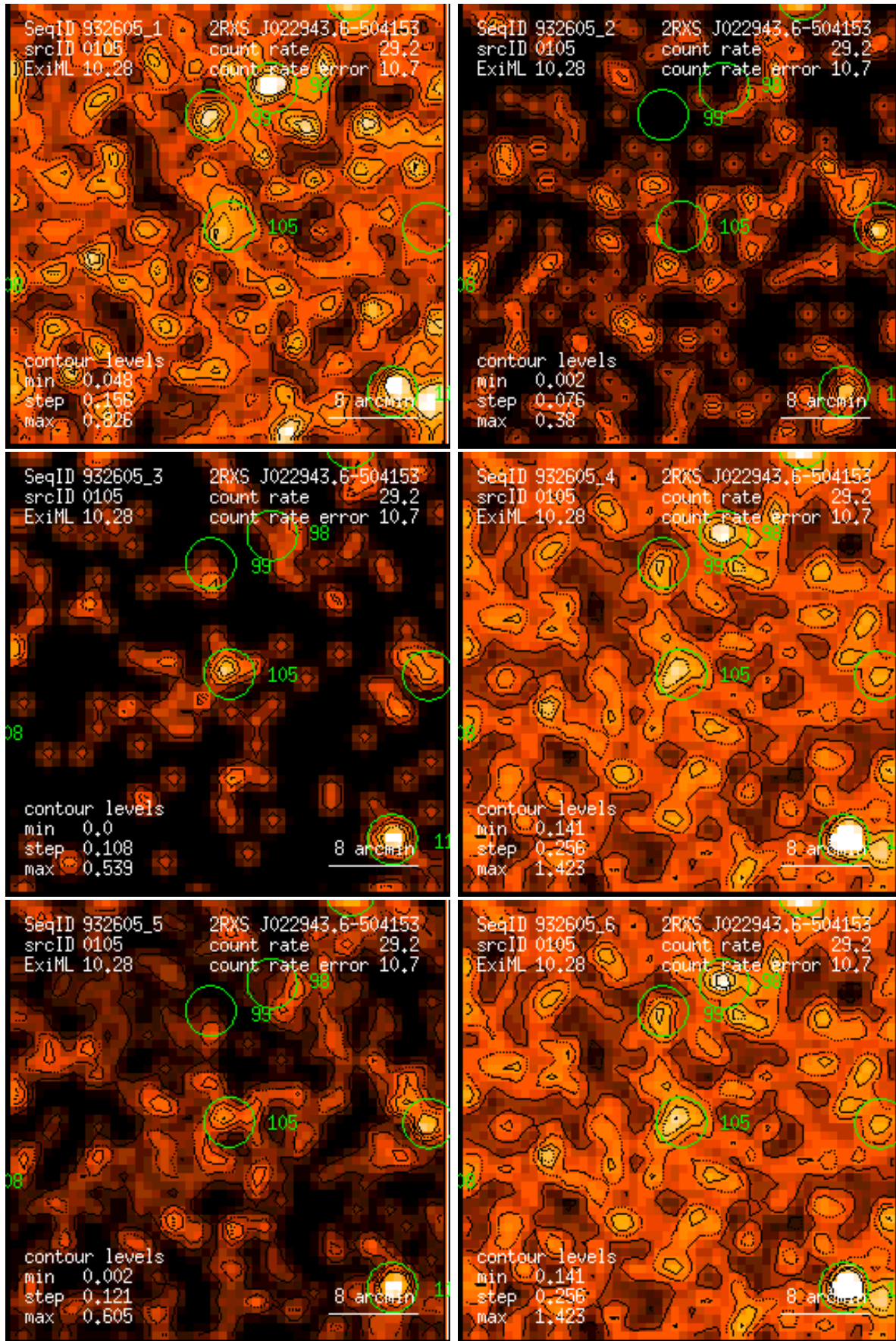
Figure 105: RASS 932605: detection 0105: band rate images, Gaussian filter: (1) PSPC channels 11 – 41, (2) 52 – 90, (3) 91 – 201, (4) 11 – 235, (5) 52 – 201, (6) 11 – 201. Broad band rates in counts/ks. Band rate contour levels in counts/ks/arcmin 2 .
