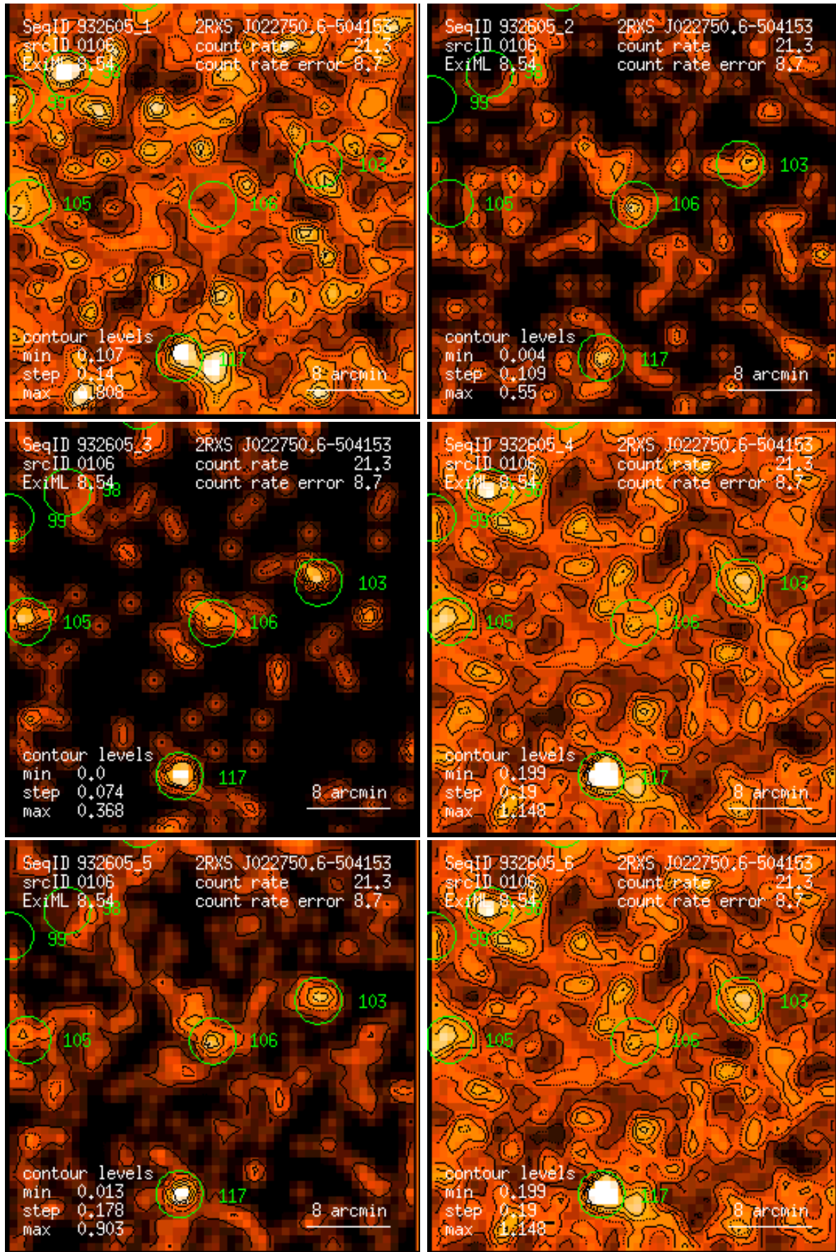
Figure 106: RASS 932605: detection 0106: band rate images, Gaussian filter: (1) PSPC channels 11 – 41, (2) 52 – 90, (3) 91 – 201, (4) 11 – 235, (5) 52 – 201, (6) 11 – 201. Broad band rates in counts/ks. Band rate contour levels in counts/ks/arcmin 2 .
