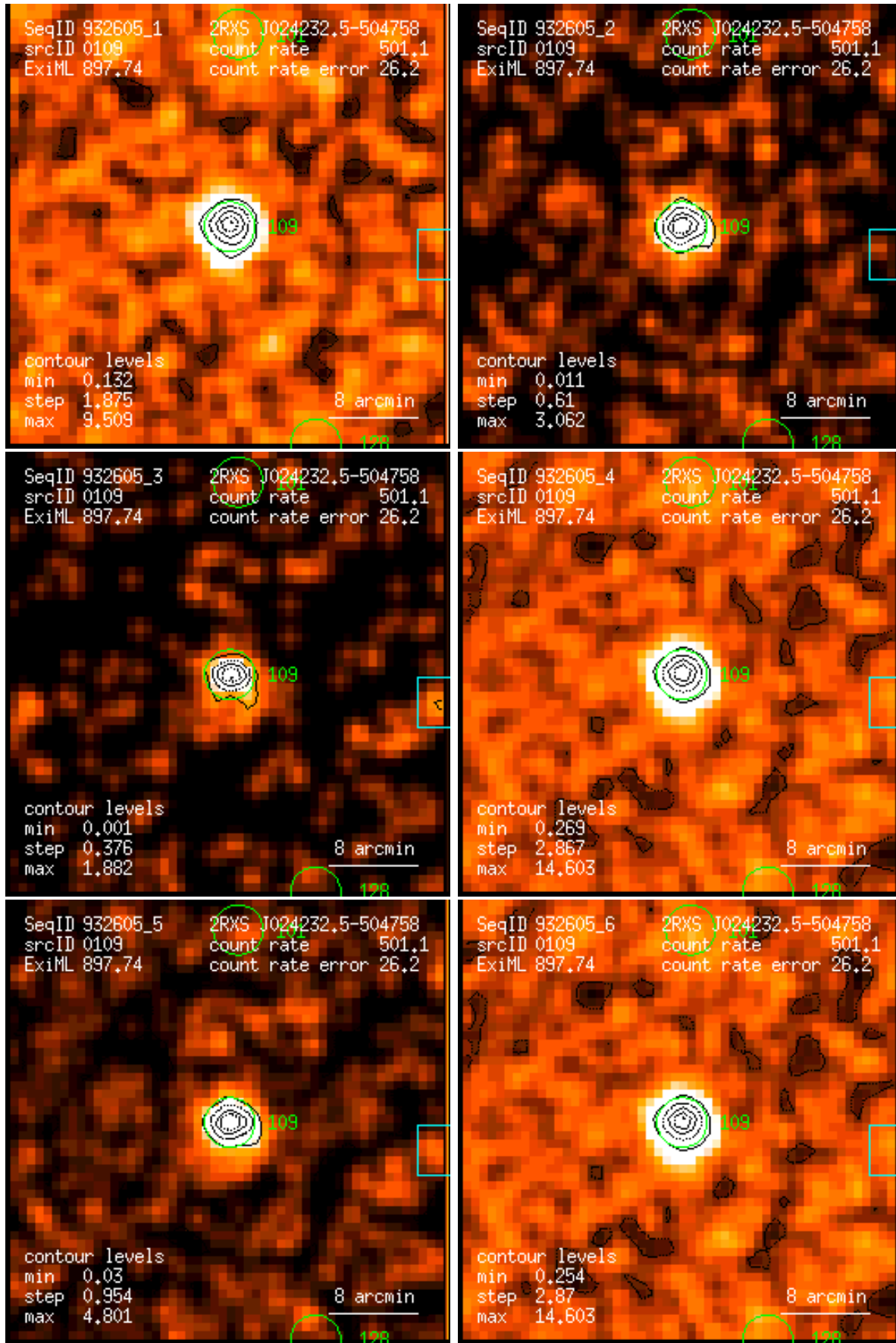
Figure 109: RASS 932605: detection 0109: band rate images, Gaussian filter: (1) PSPC channels 11 – 41, (2) 52 – 90, (3) 91 – 201, (4) 11 – 235, (5) 52 – 201, (6) 11 – 201. Broad band rates in counts/ks. Band rate contour levels in counts/ks/arcmin 2 .
