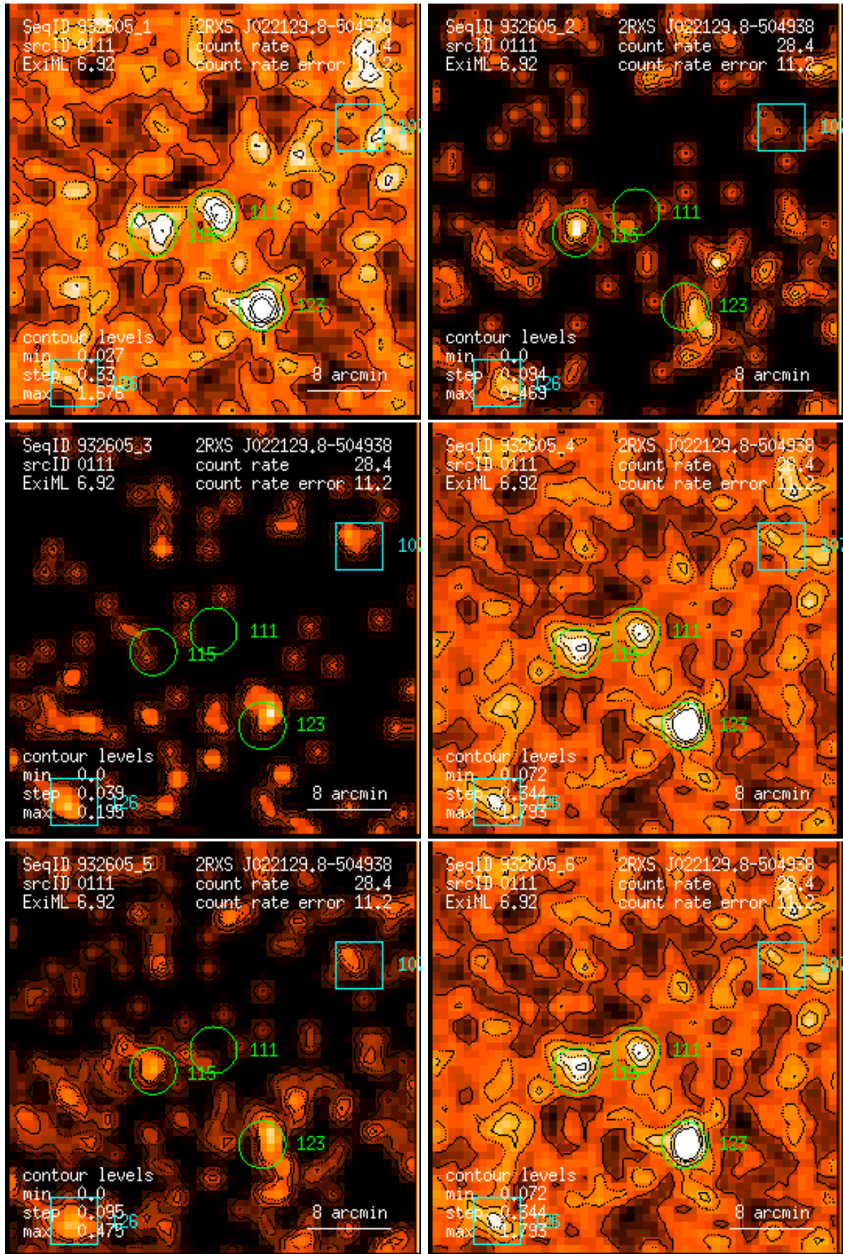
Figure 111: RASS 932605: detection 0111: band rate images, Gaussian filter: (1) PSPC channels 11 – 41, (2) 52 – 90, (3) 91 – 201, (4) 11 – 235, (5) 52 – 201, (6) 11 – 201. Broad band rates in counts/ks. Band rate contour levels in counts/ks/arcmin 2 .
