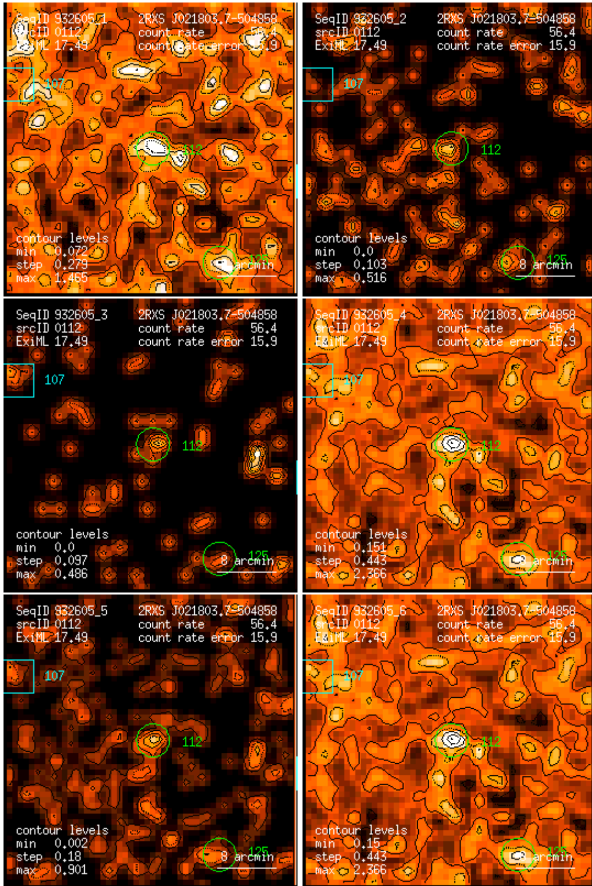
Figure 112: RASS 932605: detection 0112: band rate images, Gaussian filter: (1) PSPC channels 11 – 41, (2) 52 – 90, (3) 91 – 201, (4) 11 – 235, (5) 52 – 201, (6) 11 – 201. Broad band rates in counts/ks. Band rate contour levels in counts/ks/arcmin 2 .
