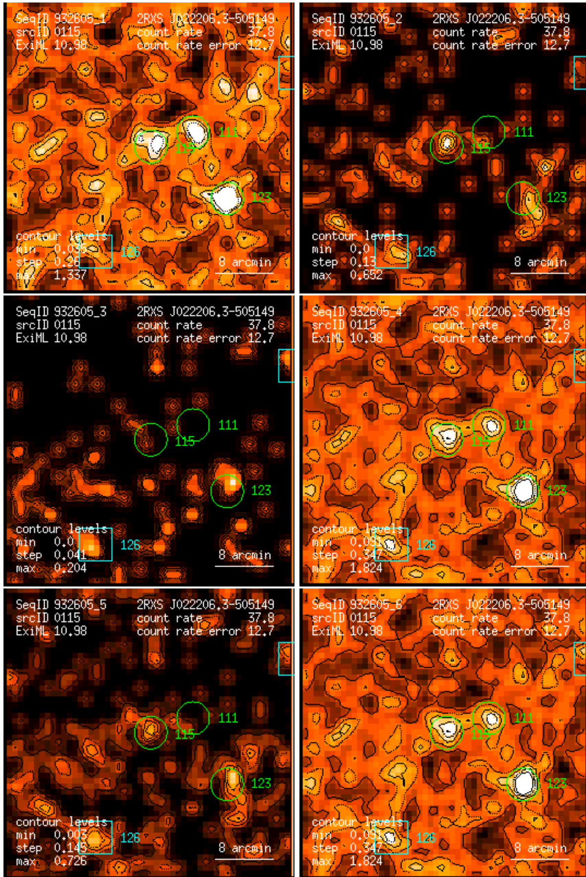
Figure 115: RASS 932605: detection 0115: band rate images, Gaussian filter: (1) PSPC channels 11 – 41, (2) 52 – 90, (3) 91 – 201, (4) 11 – 235, (5) 52 – 201, (6) 11 – 201. Broad band rates in counts/ks. Band rate contour levels in counts/ks/arcmin 2 .
