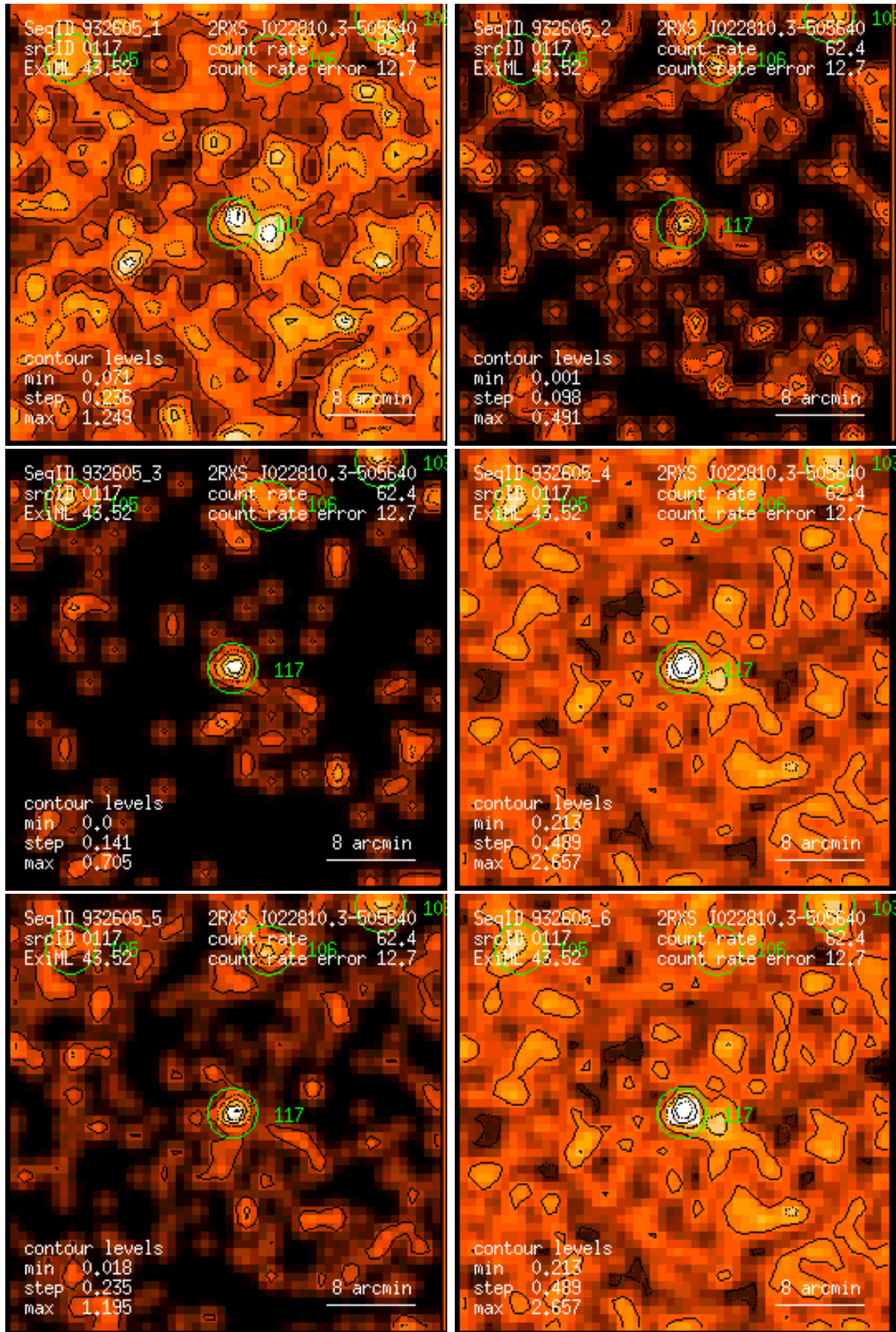
Figure 117: RASS 932605: detection 0117: band rate images, Gaussian filter: (1) PSPC channels 11 – 41, (2) 52 – 90, (3) 91 – 201, (4) 11 – 235, (5) 52 – 201, (6) 11 – 201. Broad band rates in counts/ks. Band rate contour levels in counts/ks/arcmin 2 .
