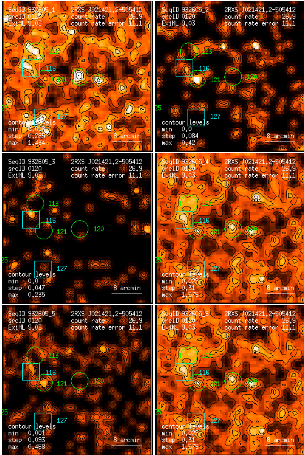
Figure 120: RASS 932605: detection 0120: band rate images, Gaussian filter: (1) PSPC channels 11 – 41, (2) 52 – 90, (3) 91 – 201, (4) 11 – 235, (5) 52 – 201, (6) 11 – 201. Broad band rates in counts/ks. Band rate contour levels in counts/ks/arcmin 2 .
