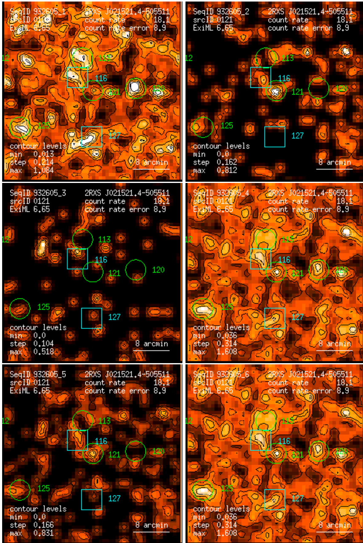
Figure 121: RASS 932605: detection 0121: band rate images, Gaussian filter: (1) PSPC channels 11 – 41, (2) 52 – 90, (3) 91 – 201, (4) 11 – 235, (5) 52 – 201, (6) 11 – 201. Broad band rates in counts/ks. Band rate contour levels in counts/ks/arcmin 2 .
