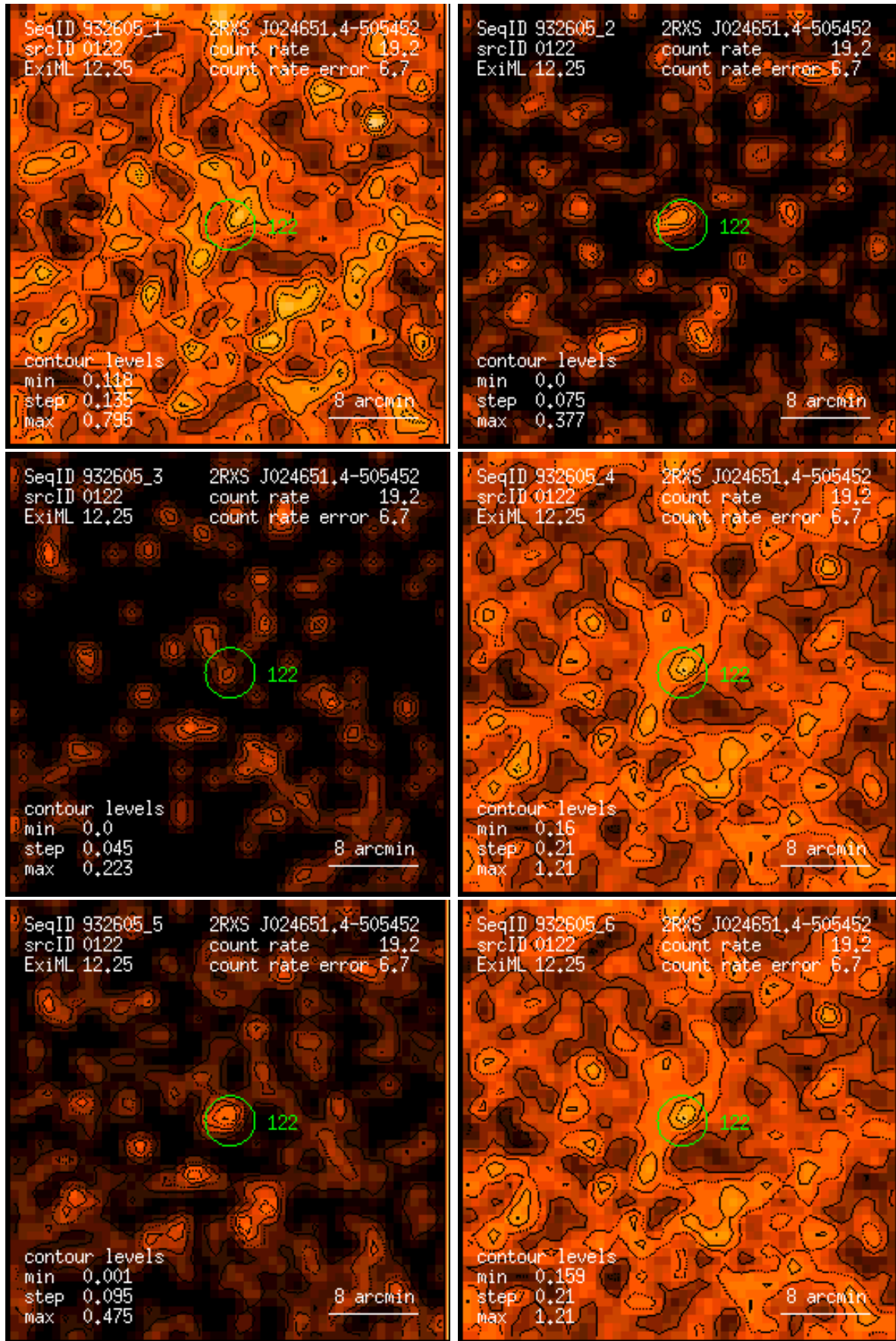
Figure 122: RASS 932605: detection 0122: band rate images, Gaussian filter: (1) PSPC channels 11 – 41, (2) 52 – 90, (3) 91 – 201, (4) 11 – 235, (5) 52 – 201, (6) 11 – 201. Broad band rates in counts/ks. Band rate contour levels in counts/ks/arcmin 2 .
