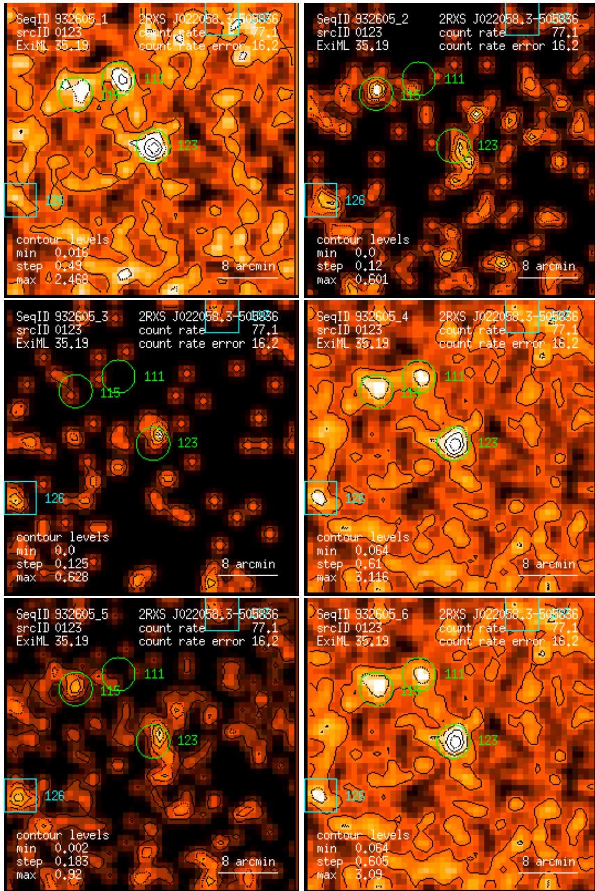
Figure 123: RASS 932605: detection 0123: band rate images, Gaussian filter: (1) PSPC channels 11 – 41, (2) 52 – 90, (3) 91 – 201, (4) 11 – 235, (5) 52 – 201, (6) 11 – 201. Broad band rates in counts/ks. Band rate contour levels in counts/ks/arcmin 2 .
