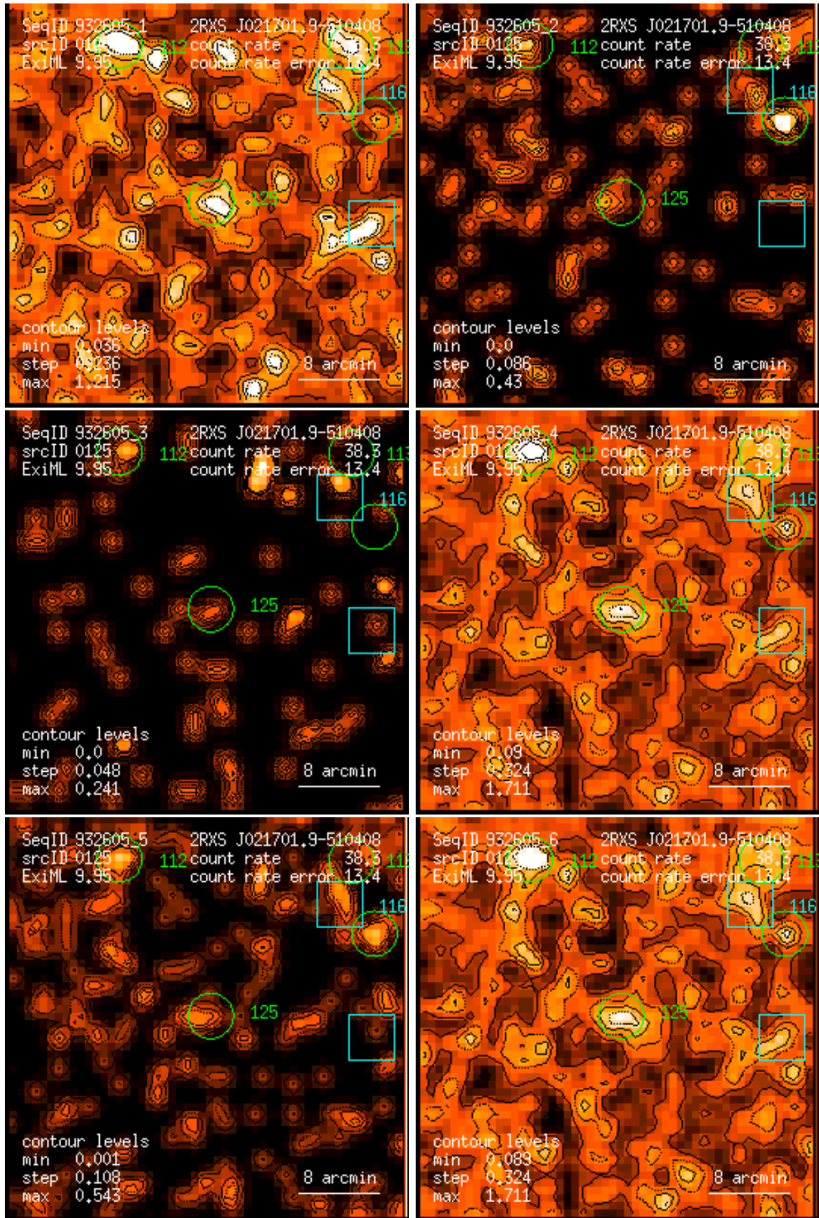
Figure 125: RASS 932605: detection 0125: band rate images, Gaussian filter: (1) PSPC channels 11 – 41, (2) 52 – 90, (3) 91 – 201, (4) 11 – 235, (5) 52 – 201, (6) 11 – 201. Broad band rates in counts/ks. Band rate contour levels in counts/ks/arcmin 2 .
