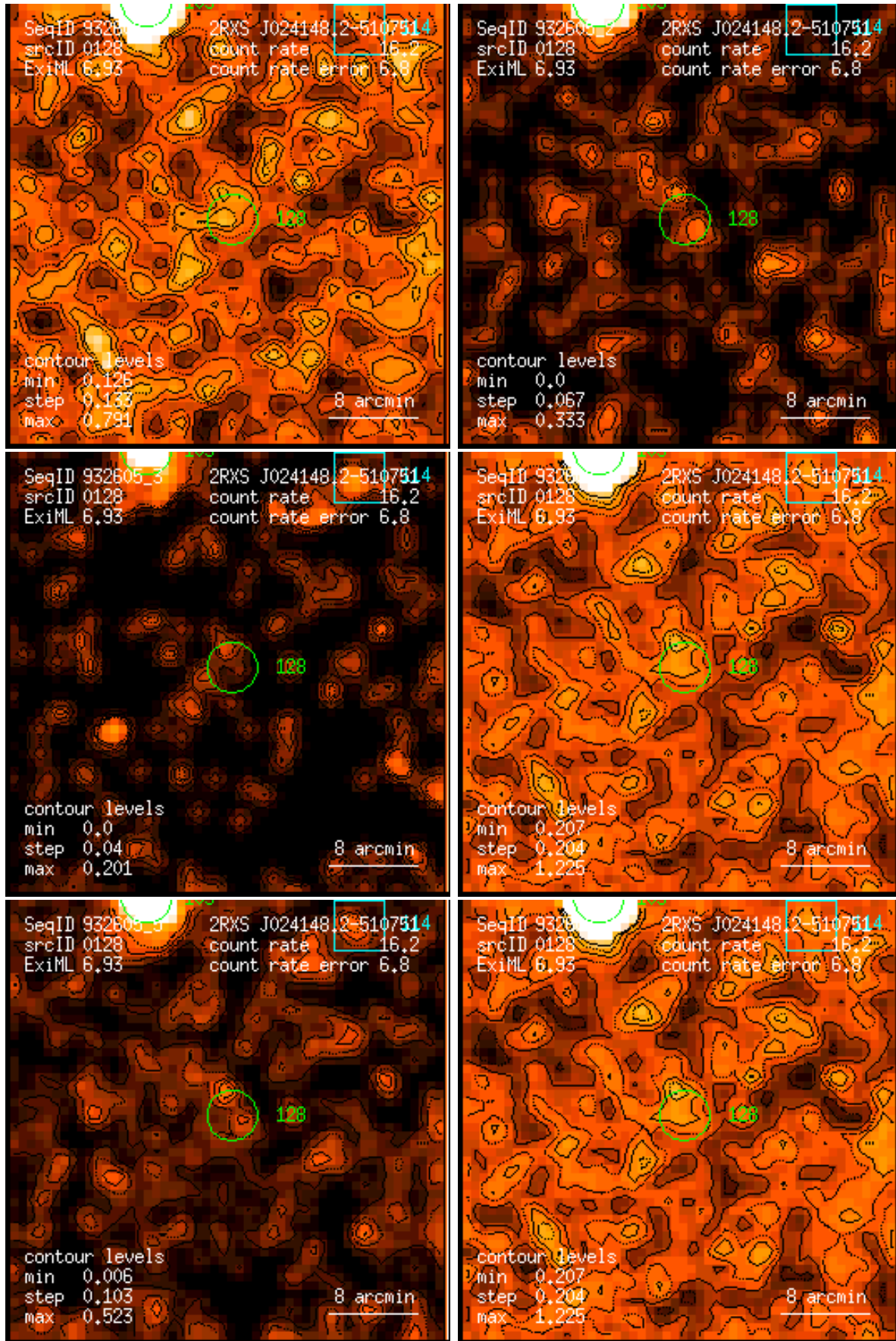
Figure 128: RASS 932605: detection 0128: band rate images, Gaussian filter: (1) PSPC channels 11 – 41, (2) 52 – 90, (3) 91 – 201, (4) 11 – 235, (5) 52 – 201, (6) 11 – 201. Broad band rates in counts/ks. Band rate contour levels in counts/ks/arcmin 2 .
