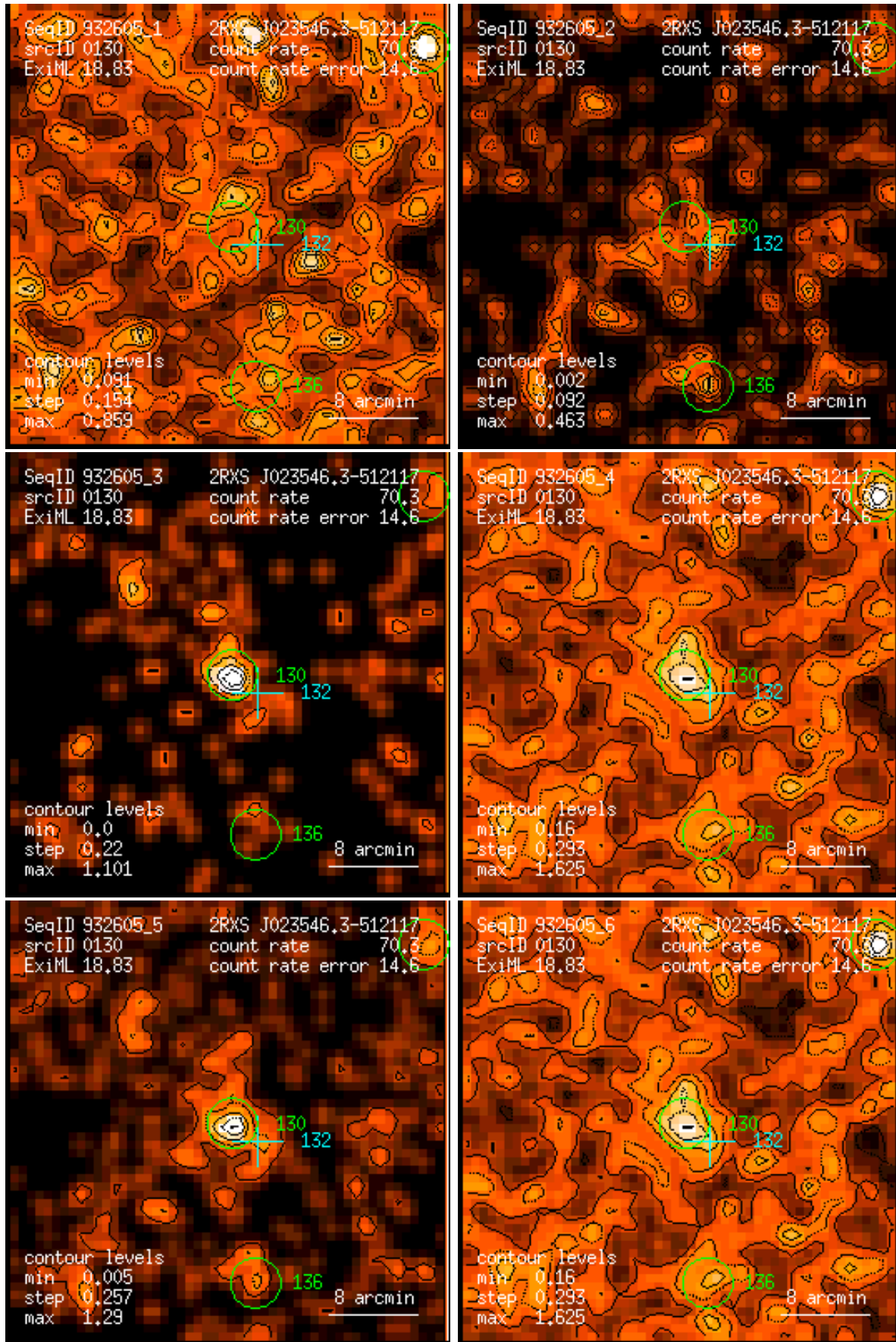
Figure 130: RASS 932605: detection 0130: band rate images, Gaussian filter: (1) PSPC channels 11 – 41, (2) 52 – 90, (3) 91 – 201, (4) 11 – 235, (5) 52 – 201, (6) 11 – 201. Broad band rates in counts/ks. Band rate contour levels in counts/ks/arcmin 2 .
