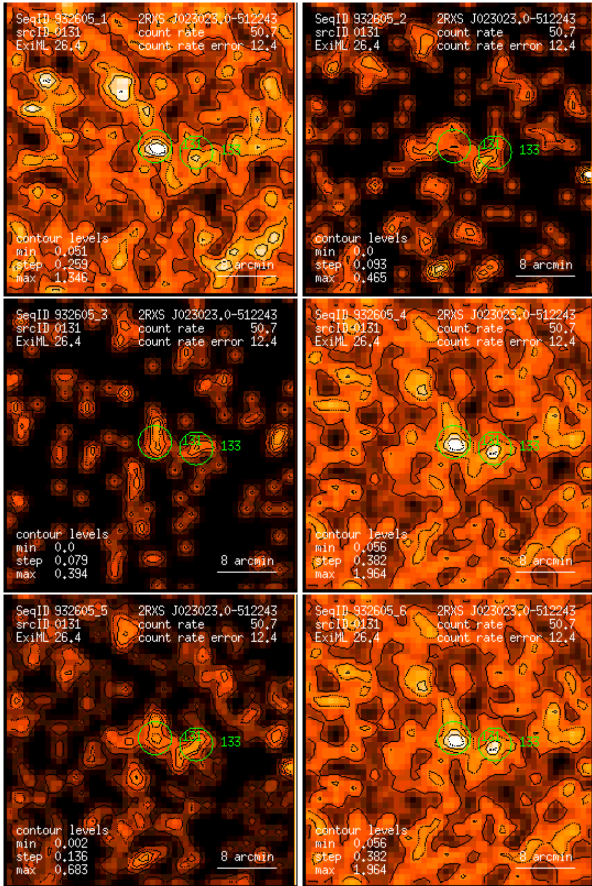
Figure 131: RASS 932605: detection 0131: band rate images, Gaussian filter: (1) PSPC channels 11 – 41, (2) 52 – 90, (3) 91 – 201, (4) 11 – 235, (5) 52 – 201, (6) 11 – 201. Broad band rates in counts/ks. Band rate contour levels in counts/ks/arcmin 2 .
