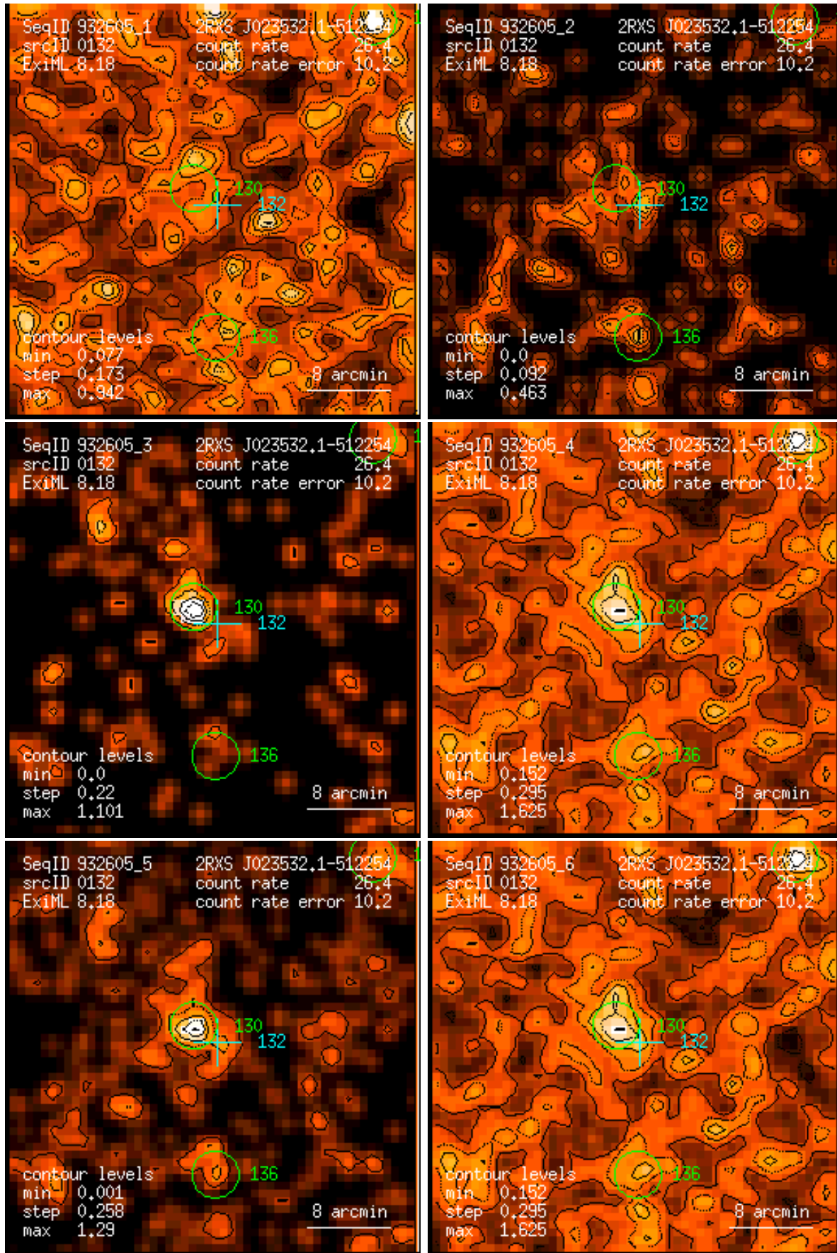
Figure 132: RASS 932605: detection 0132: band rate images, Gaussian filter: (1) PSPC channels 11 – 41, (2) 52 – 90, (3) 91 – 201, (4) 11 – 235, (5) 52 – 201, (6) 11 – 201. Broad band rates in counts/ks. Band rate contour levels in counts/ks/arcmin 2 .
