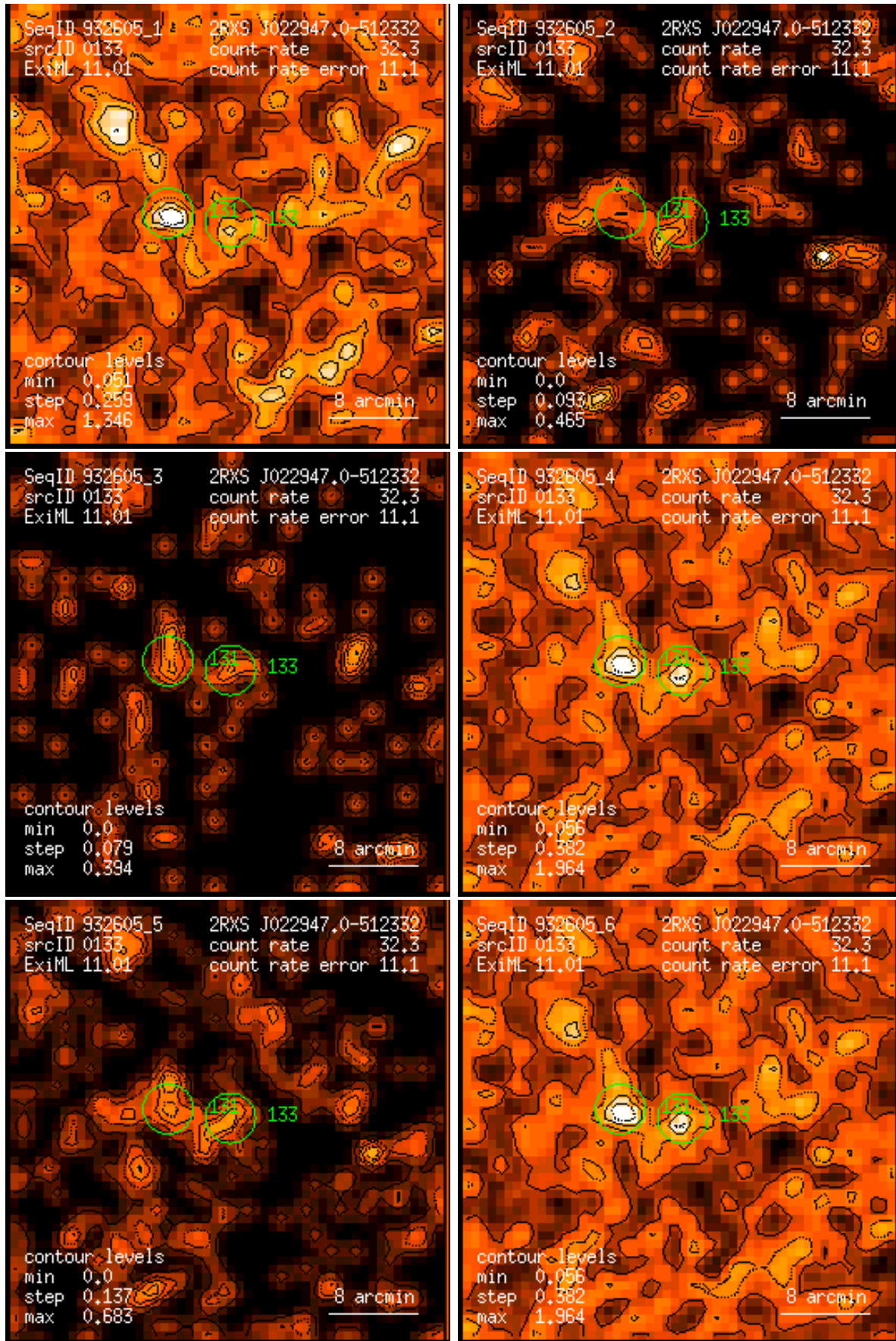
Figure 133: RASS 932605: detection 0133: band rate images, Gaussian filter: (1) PSPC channels 11 – 41, (2) 52 – 90, (3) 91 – 201, (4) 11 – 235, (5) 52 – 201, (6) 11 – 201. Broad band rates in counts/ks. Band rate contour levels in counts/ks/arcmin 2 .
