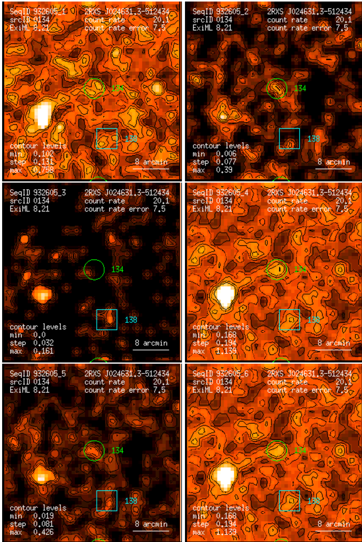
Figure 134: RASS 932605: detection 0134: band rate images, Gaussian filter: (1) PSPC channels 11 – 41, (2) 52 – 90, (3) 91 – 201, (4) 11 – 235, (5) 52 – 201, (6) 11 – 201. Broad band rates in counts/ks. Band rate contour levels in counts/ks/arcmin 2 .
