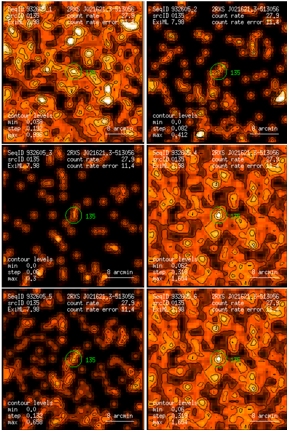
Figure 135: RASS 932605: detection 0135: band rate images, Gaussian filter: (1) PSPC channels 11 – 41, (2) 52 – 90, (3) 91 – 201, (4) 11 – 235, (5) 52 – 201, (6) 11 – 201. Broad band rates in counts/ks. Band rate contour levels in counts/ks/arcmin 2 .
