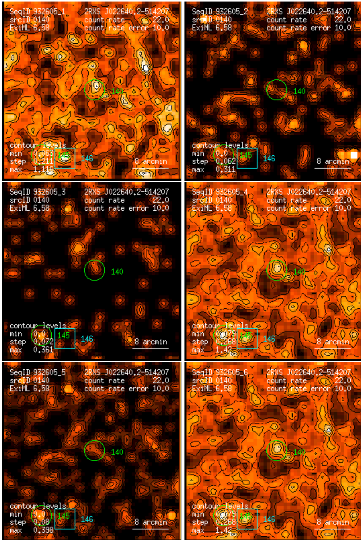
Figure 140: RASS 932605: detection 0140: band rate images, Gaussian filter: (1) PSPC channels 11 – 41, (2) 52 – 90, (3) 91 – 201, (4) 11 – 235, (5) 52 – 201, (6) 11 – 201. Broad band rates in counts/ks. Band rate contour levels in counts/ks/arcmin 2 .
