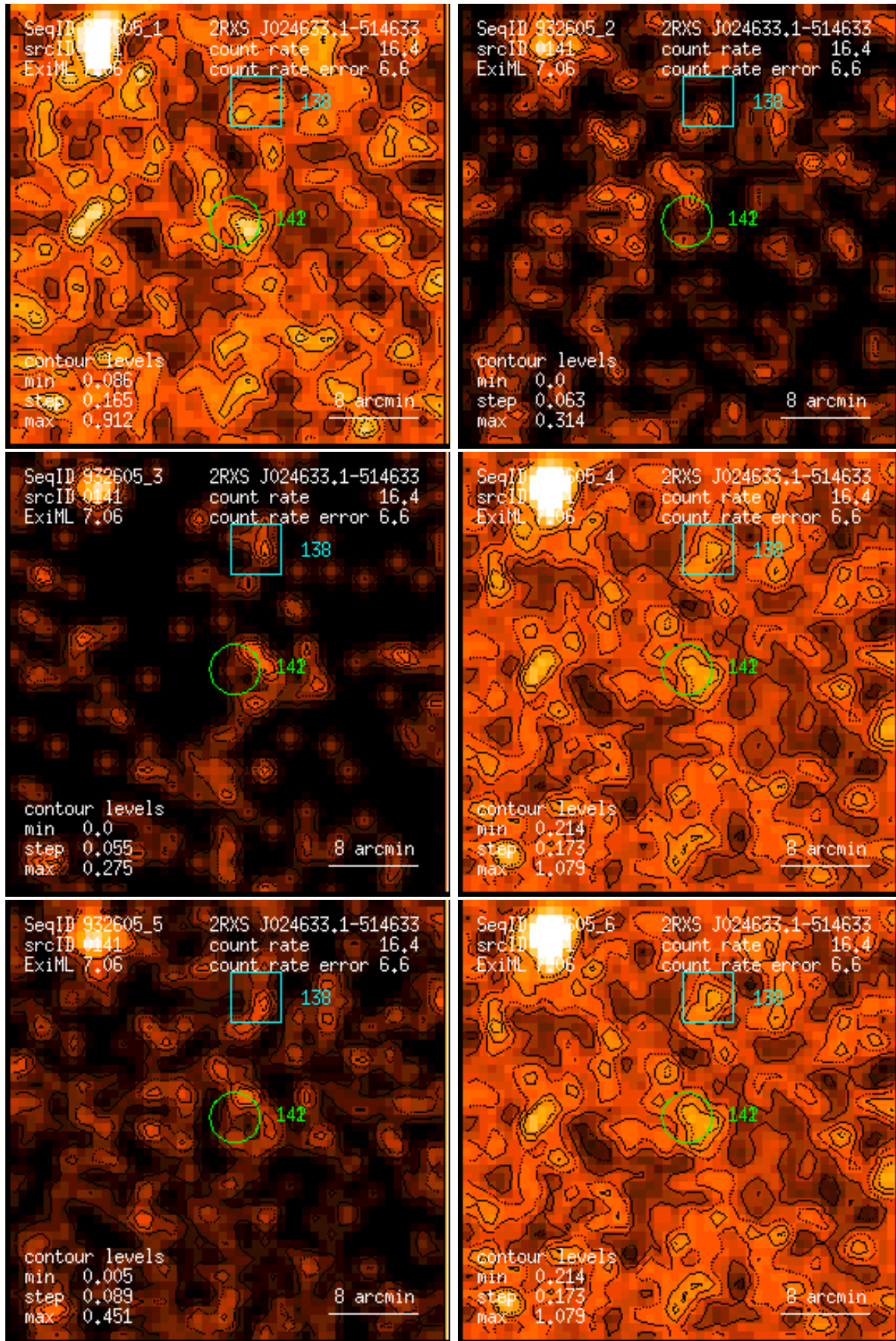
Figure 141: RASS 932605: detection 0141: band rate images, Gaussian filter: (1) PSPC channels 11 – 41, (2) 52 – 90, (3) 91 – 201, (4) 11 – 235, (5) 52 – 201, (6) 11 – 201. Broad band rates in counts/ks. Band rate contour levels in counts/ks/arcmin 2 .
