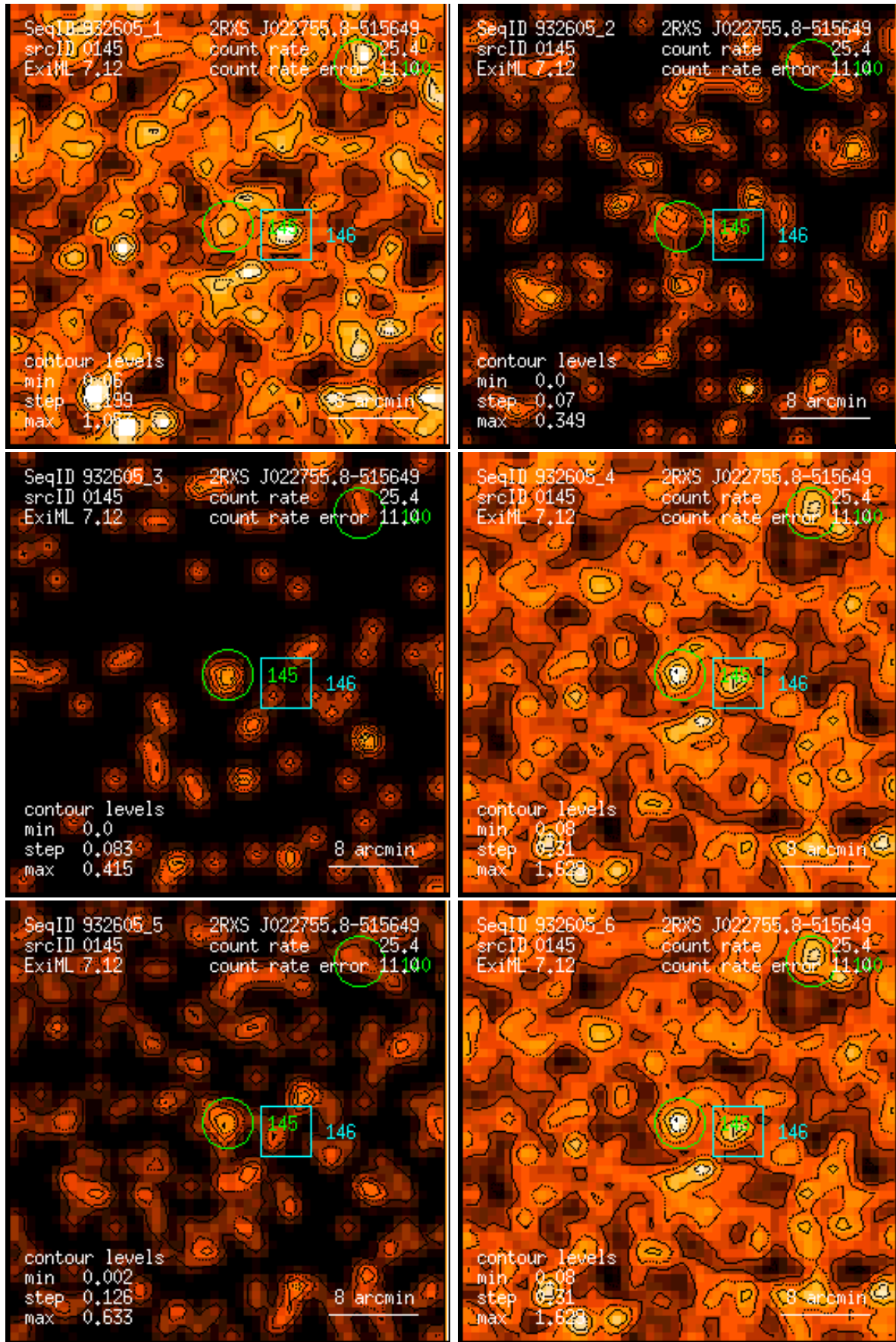
Figure 145: RASS 932605: detection 0145: band rate images, Gaussian filter: (1) PSPC channels 11 – 41, (2) 52 – 90, (3) 91 – 201, (4) 11 – 235, (5) 52 – 201, (6) 11 – 201. Broad band rates in counts/ks. Band rate contour levels in counts/ks/arcmin 2 .
