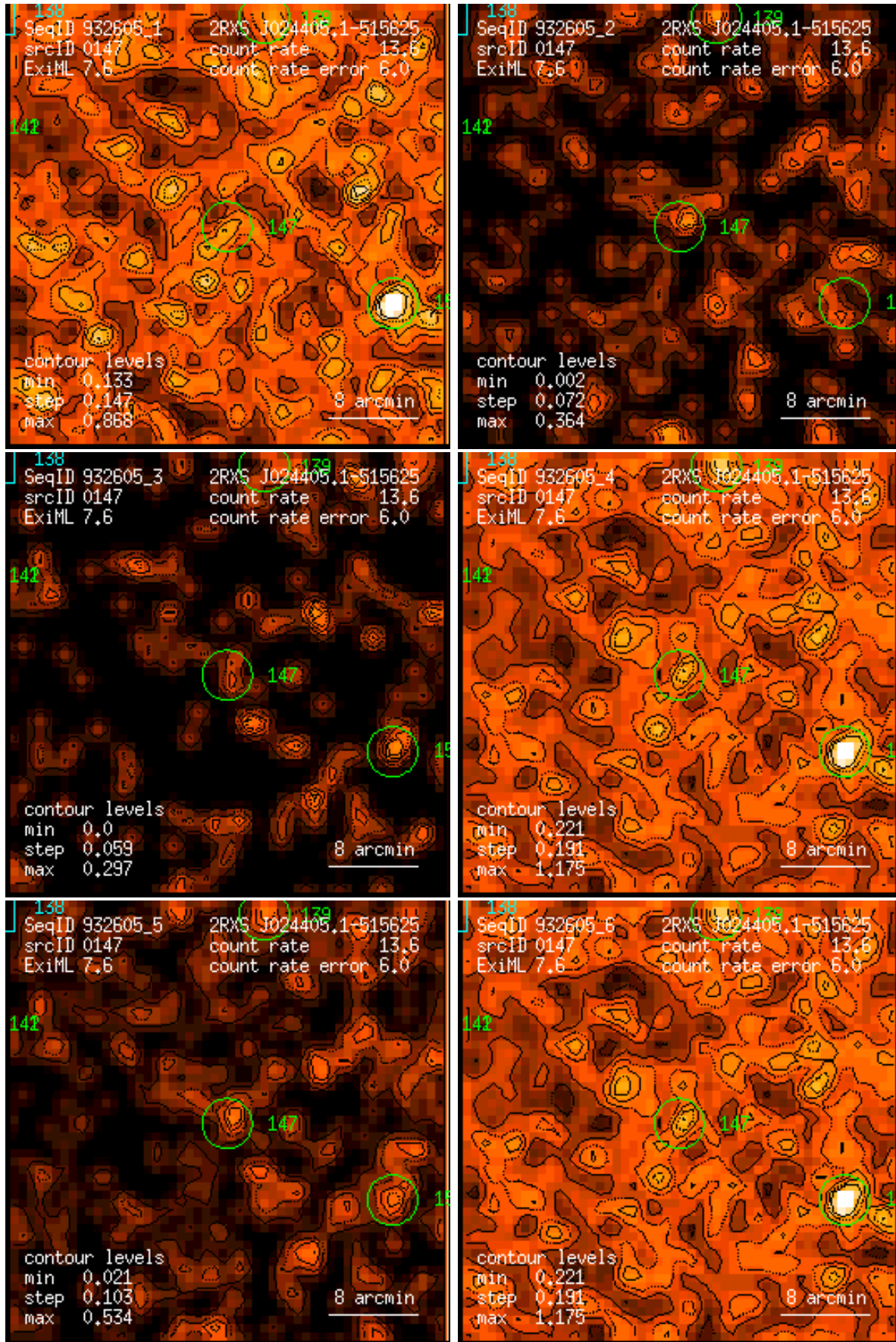
Figure 147: RASS 932605: detection 0147: band rate images, Gaussian filter: (1) PSPC channels 11 – 41, (2) 52 – 90, (3) 91 – 201, (4) 11 – 235, (5) 52 – 201, (6) 11 – 201. Broad band rates in counts/ks. Band rate contour levels in counts/ks/arcmin 2 .
