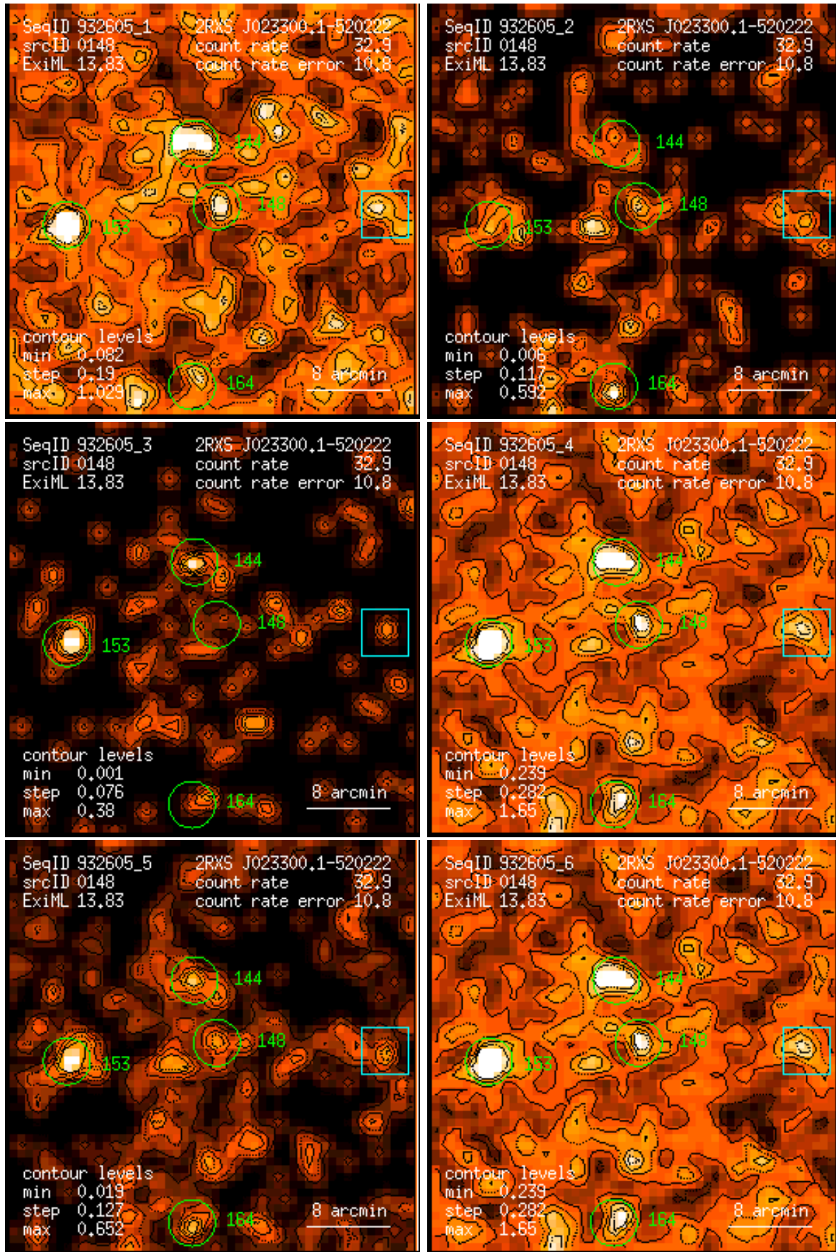
Figure 148: RASS 932605: detection 0148: band rate images, Gaussian filter: (1) PSPC channels 11 – 41, (2) 52 – 90, (3) 91 – 201, (4) 11 – 235, (5) 52 – 201, (6) 11 – 201. Broad band rates in counts/ks. Band rate contour levels in counts/ks/arcmin 2 .
