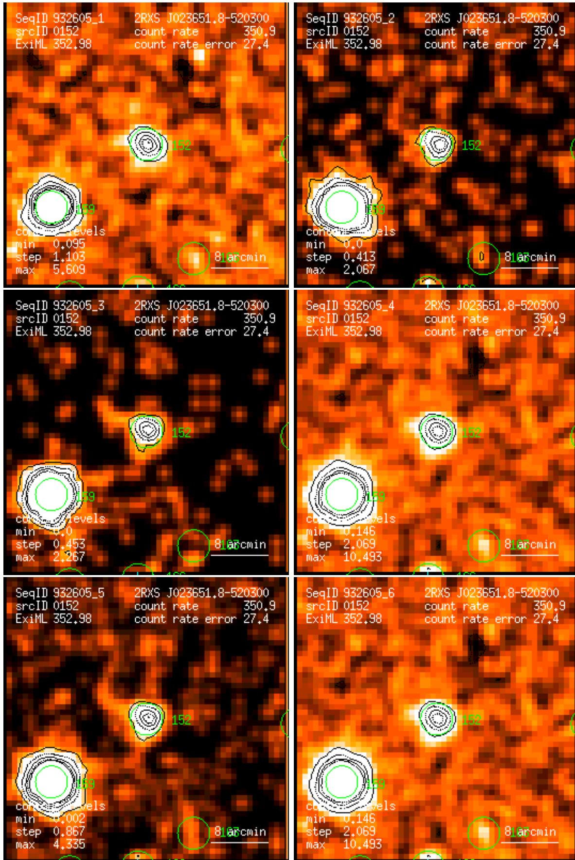
Figure 152: RASS 932605: detection 0152: band rate images, Gaussian filter: (1) PSPC channels 11 – 41, (2) 52 – 90, (3) 91 – 201, (4) 11 – 235, (5) 52 – 201, (6) 11 – 201. Broad band rates in counts/ks. Band rate contour levels in counts/ks/arcmin 2 .
