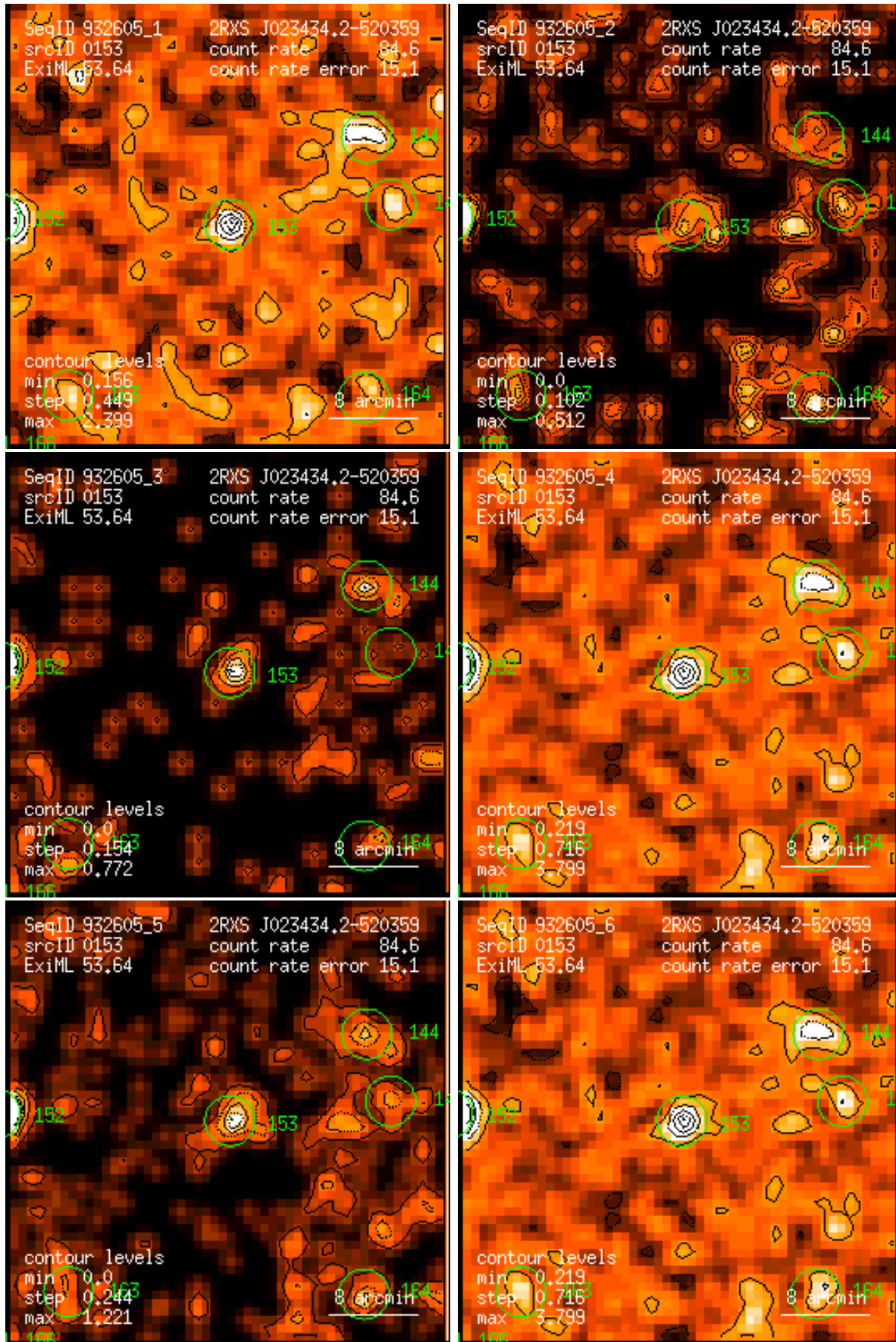
Figure 153: RASS 932605: detection 0153: band rate images, Gaussian filter: (1) PSPC channels 11 – 41, (2) 52 – 90, (3) 91 – 201, (4) 11 – 235, (5) 52 – 201, (6) 11 – 201. Broad band rates in counts/ks. Band rate contour levels in counts/ks/arcmin 2 .
