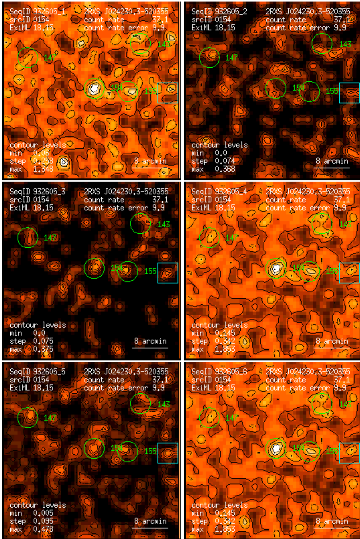
Figure 154: RASS 932605: detection 0154: band rate images, Gaussian filter: (1) PSPC channels 11 – 41, (2) 52 – 90, (3) 91 – 201, (4) 11 – 235, (5) 52 – 201, (6) 11 – 201. Broad band rates in counts/ks. Band rate contour levels in counts/ks/arcmin 2 .
