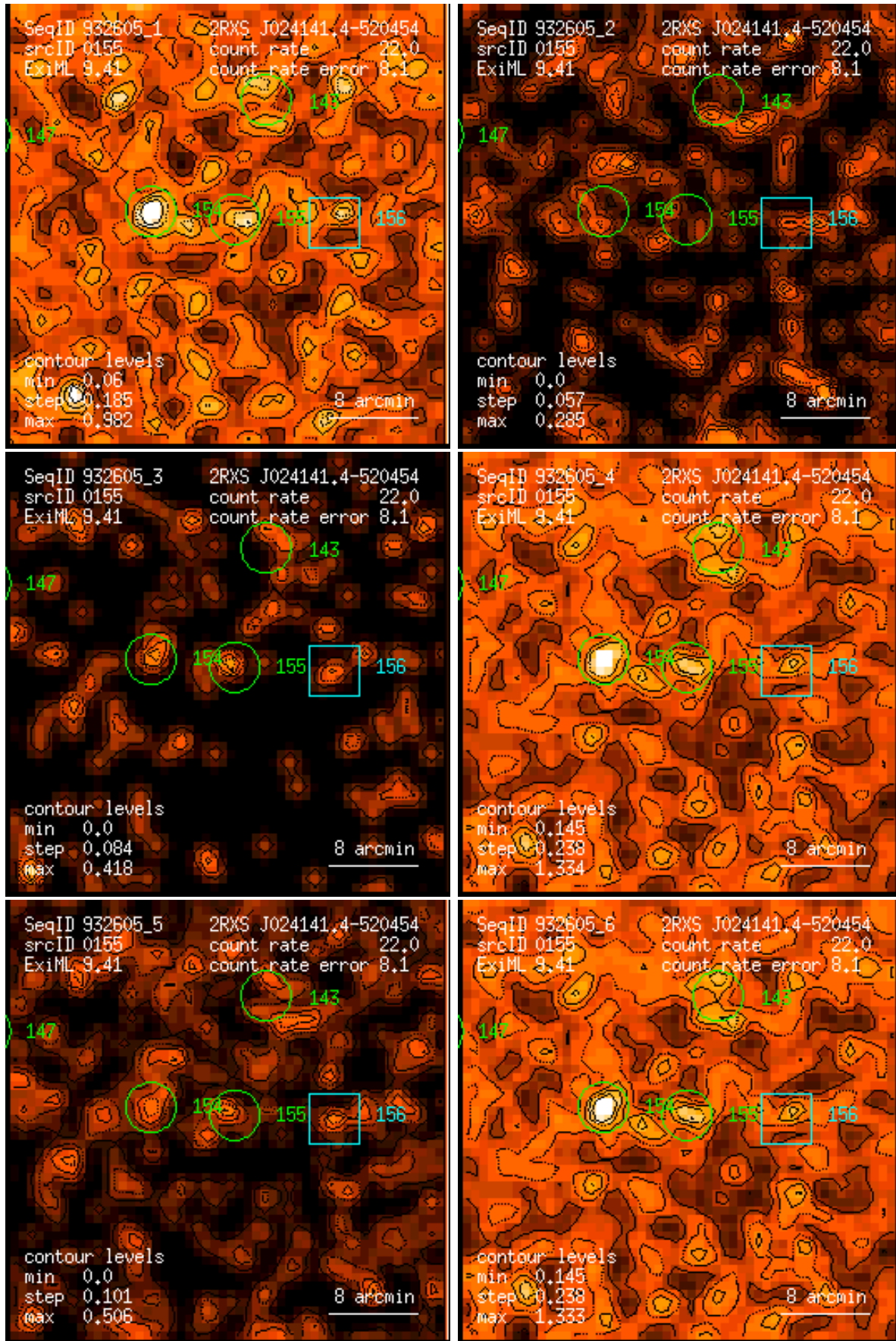
Figure 155: RASS 932605: detection 0155: band rate images, Gaussian filter: (1) PSPC channels 11 – 41, (2) 52 – 90, (3) 91 – 201, (4) 11 – 235, (5) 52 – 201, (6) 11 – 201. Broad band rates in counts/ks. Band rate contour levels in counts/ks/arcmin 2 .
