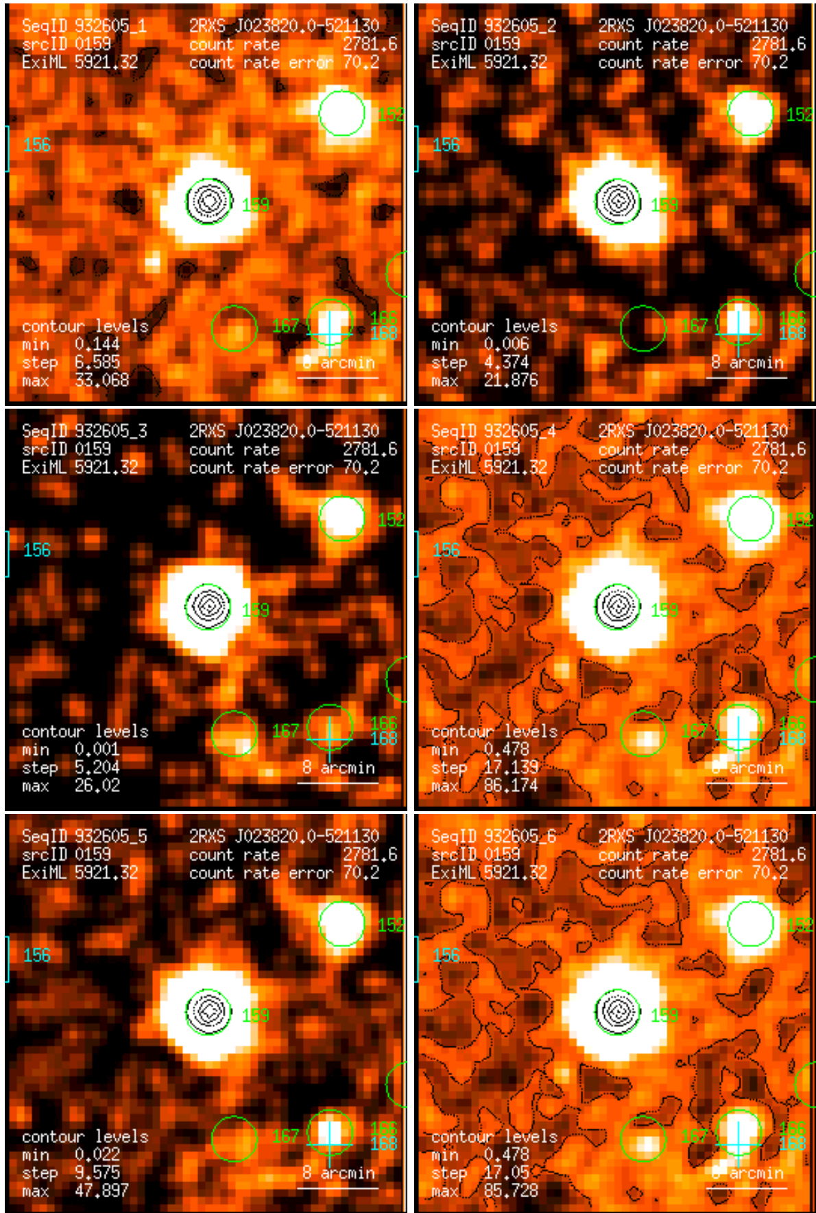
Figure 159: RASS 932605: detection 0159: band rate images, Gaussian filter: (1) PSPC channels 11 – 41, (2) 52 – 90, (3) 91 – 201, (4) 11 – 235, (5) 52 – 201, (6) 11 – 201. Broad band rates in counts/ks. Band rate contour levels in counts/ks/arcmin 2 .
