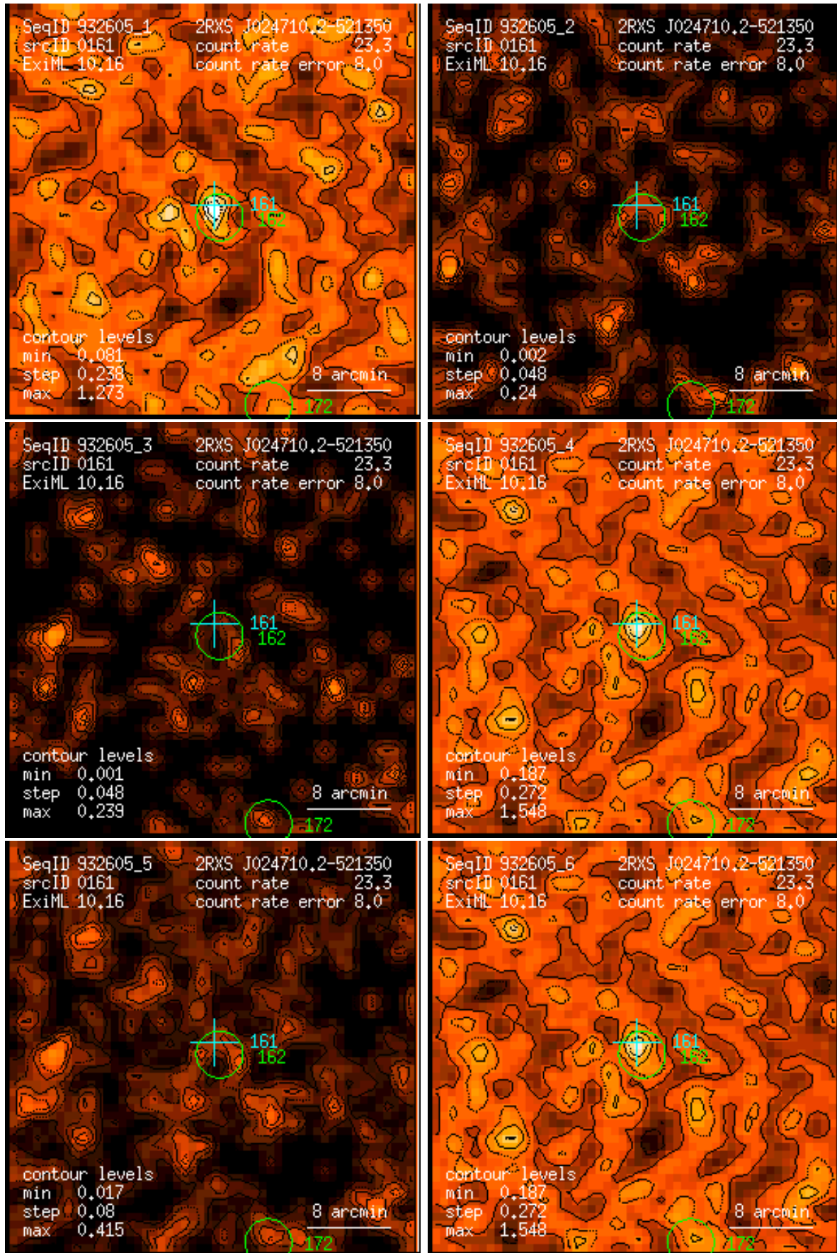
Figure 161: RASS 932605: detection 0161: band rate images, Gaussian filter: (1) PSPC channels 11 – 41, (2) 52 – 90, (3) 91 – 201, (4) 11 – 235, (5) 52 – 201, (6) 11 – 201. Broad band rates in counts/ks. Band rate contour levels in counts/ks/arcmin 2 .
