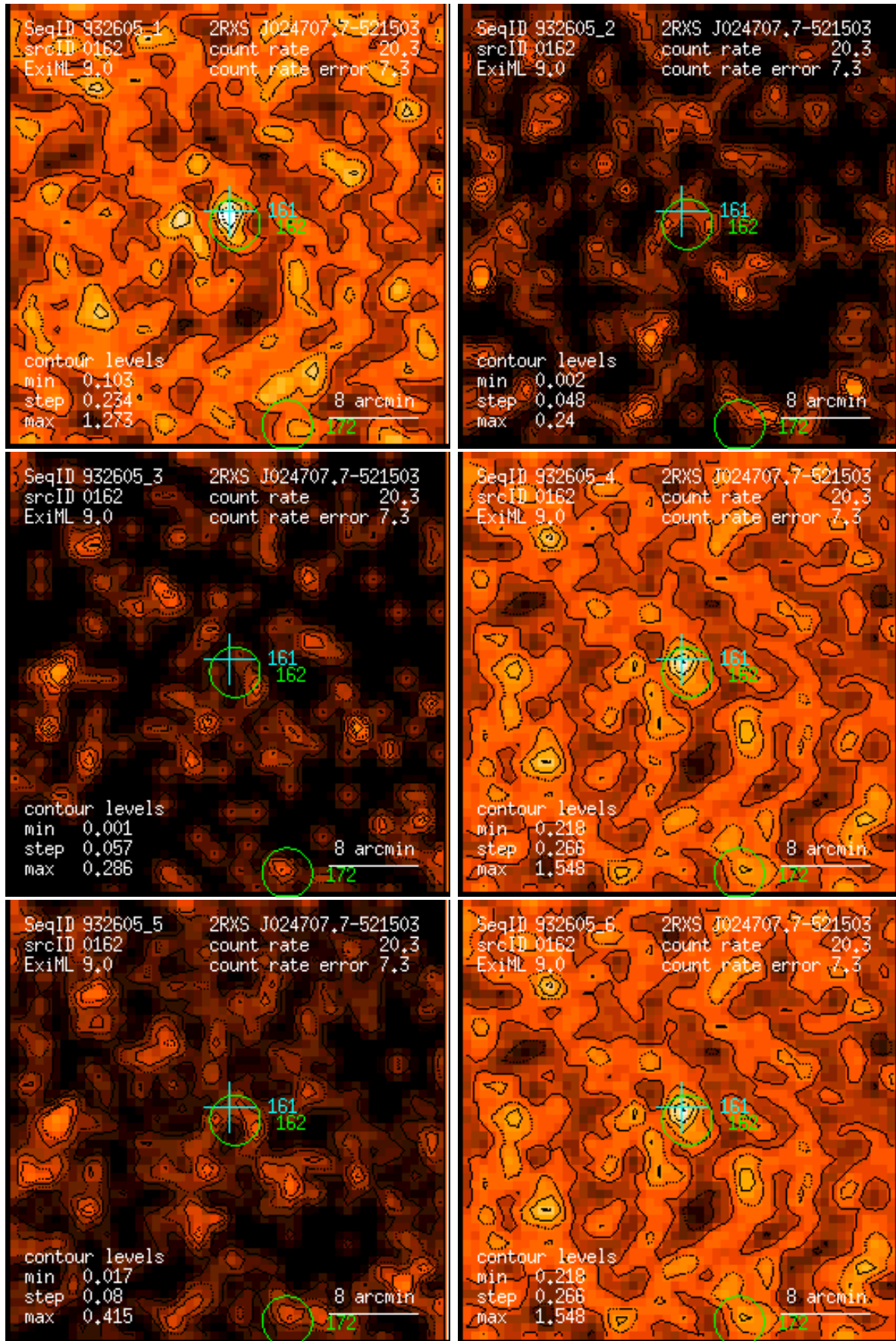
Figure 162: RASS 932605: detection 0162: band rate images, Gaussian filter: (1) PSPC channels 11 – 41, (2) 52 – 90, (3) 91 – 201, (4) 11 – 235, (5) 52 – 201, (6) 11 – 201. Broad band rates in counts/ks. Band rate contour levels in counts/ks/arcmin 2 .
