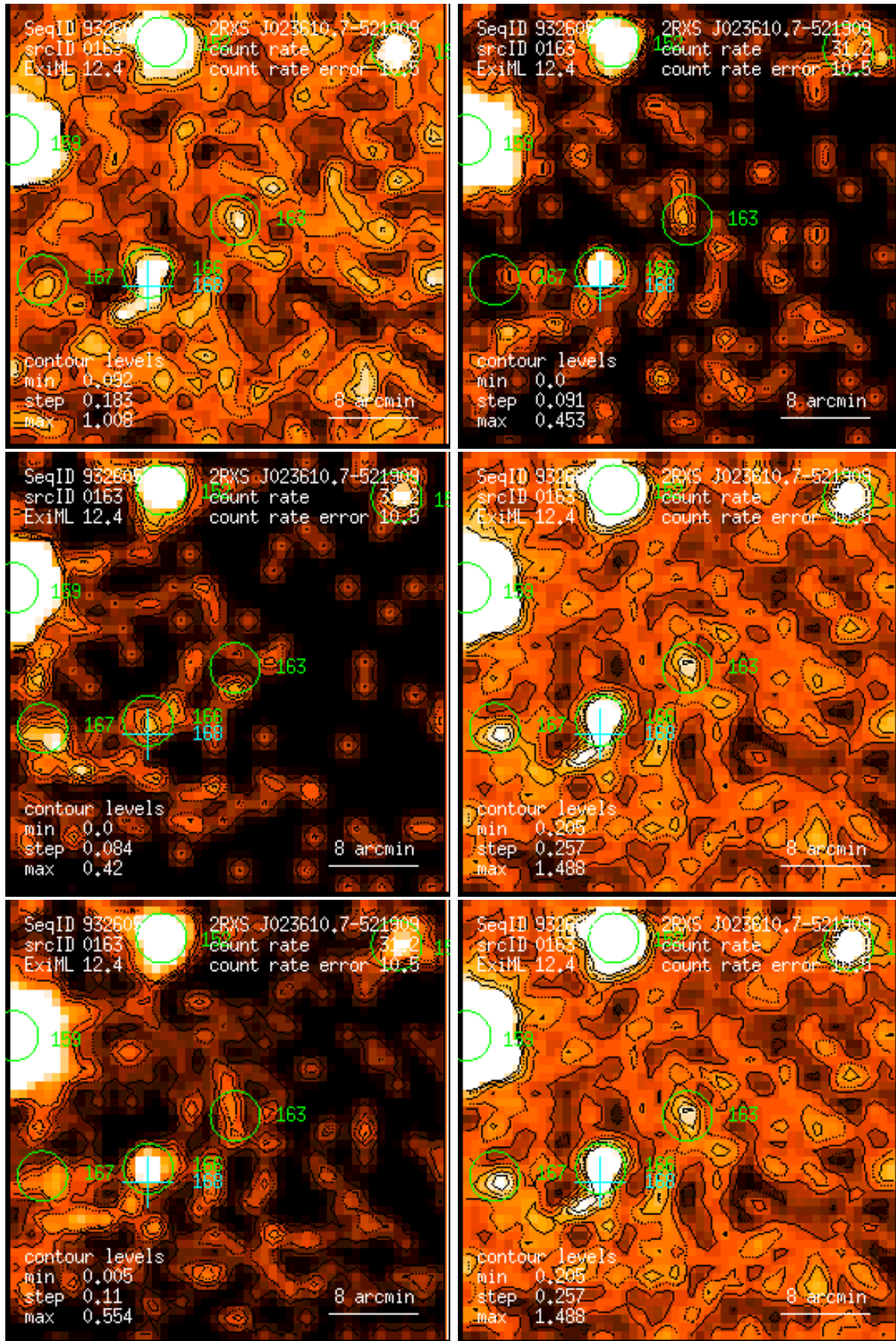
Figure 163: RASS 932605: detection 0163: band rate images, Gaussian filter: (1) PSPC channels 11 – 41, (2) 52 – 90, (3) 91 – 201, (4) 11 – 235, (5) 52 – 201, (6) 11 – 201. Broad band rates in counts/ks. Band rate contour levels in counts/ks/arcmin 2 .
