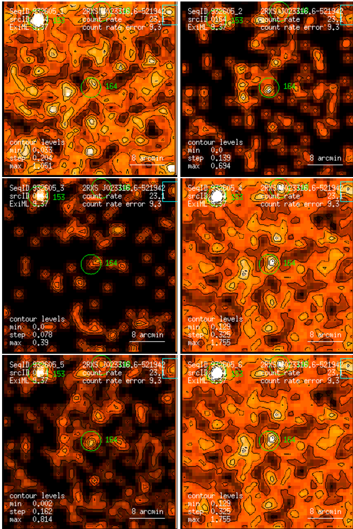
Figure 164: RASS 932605: detection 0164: band rate images, Gaussian filter: (1) PSPC channels 11 – 41, (2) 52 – 90, (3) 91 – 201, (4) 11 – 235, (5) 52 – 201, (6) 11 – 201. Broad band rates in counts/ks. Band rate contour levels in counts/ks/arcmin 2 .
