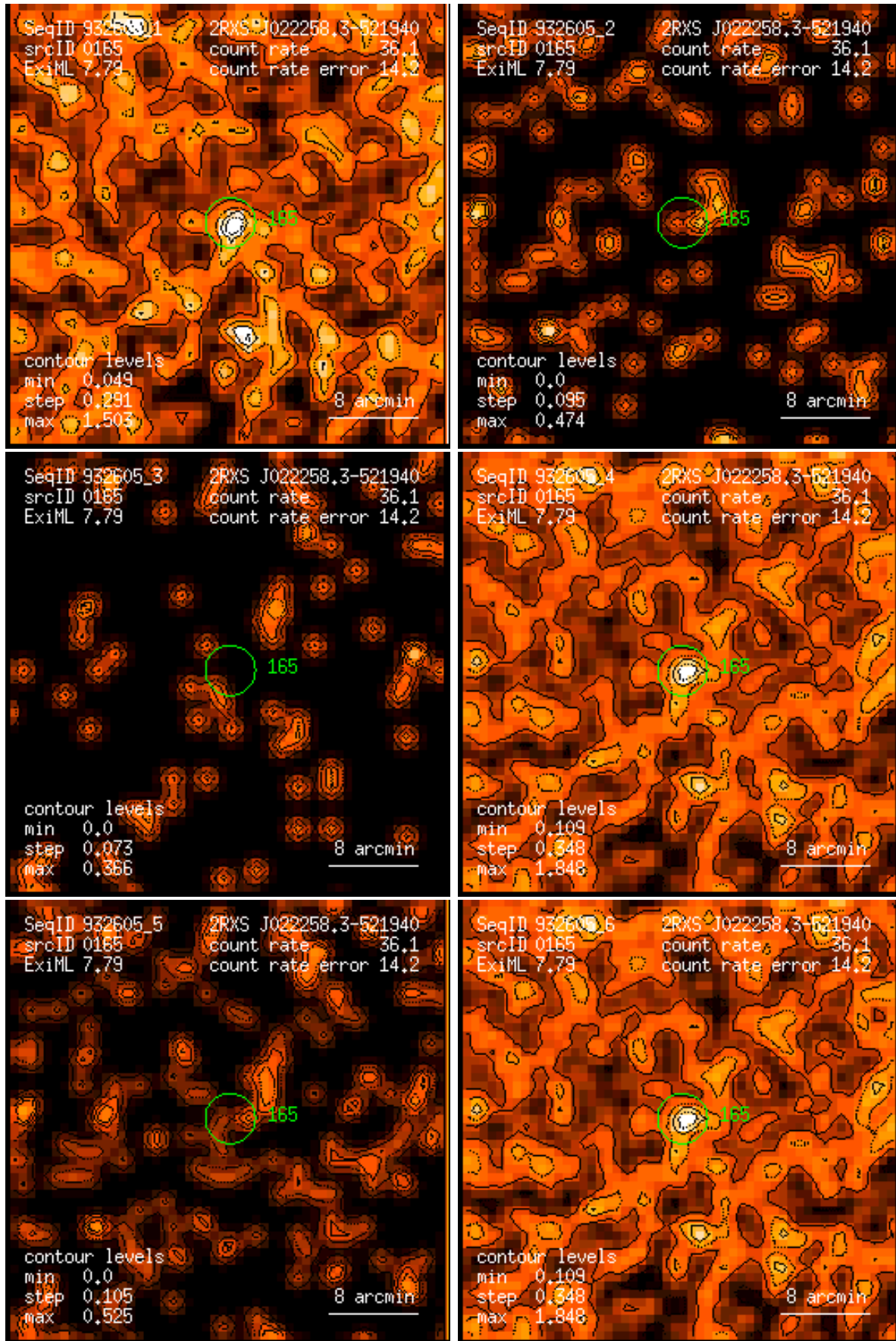
Figure 165: RASS 932605: detection 0165: band rate images, Gaussian filter: (1) PSPC channels 11 – 41, (2) 52 – 90, (3) 91 – 201, (4) 11 – 235, (5) 52 – 201, (6) 11 – 201. Broad band rates in counts/ks. Band rate contour levels in counts/ks/arcmin 2 .
