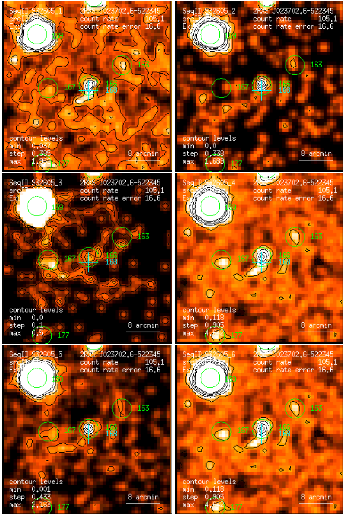
Figure 166: RASS 932605: detection 0166: band rate images, Gaussian filter: (1) PSPC channels 11 – 41, (2) 52 – 90, (3) 91 – 201, (4) 11 – 235, (5) 52 – 201, (6) 11 – 201. Broad band rates in counts/ks. Band rate contour levels in counts/ks/arcmin 2 .
