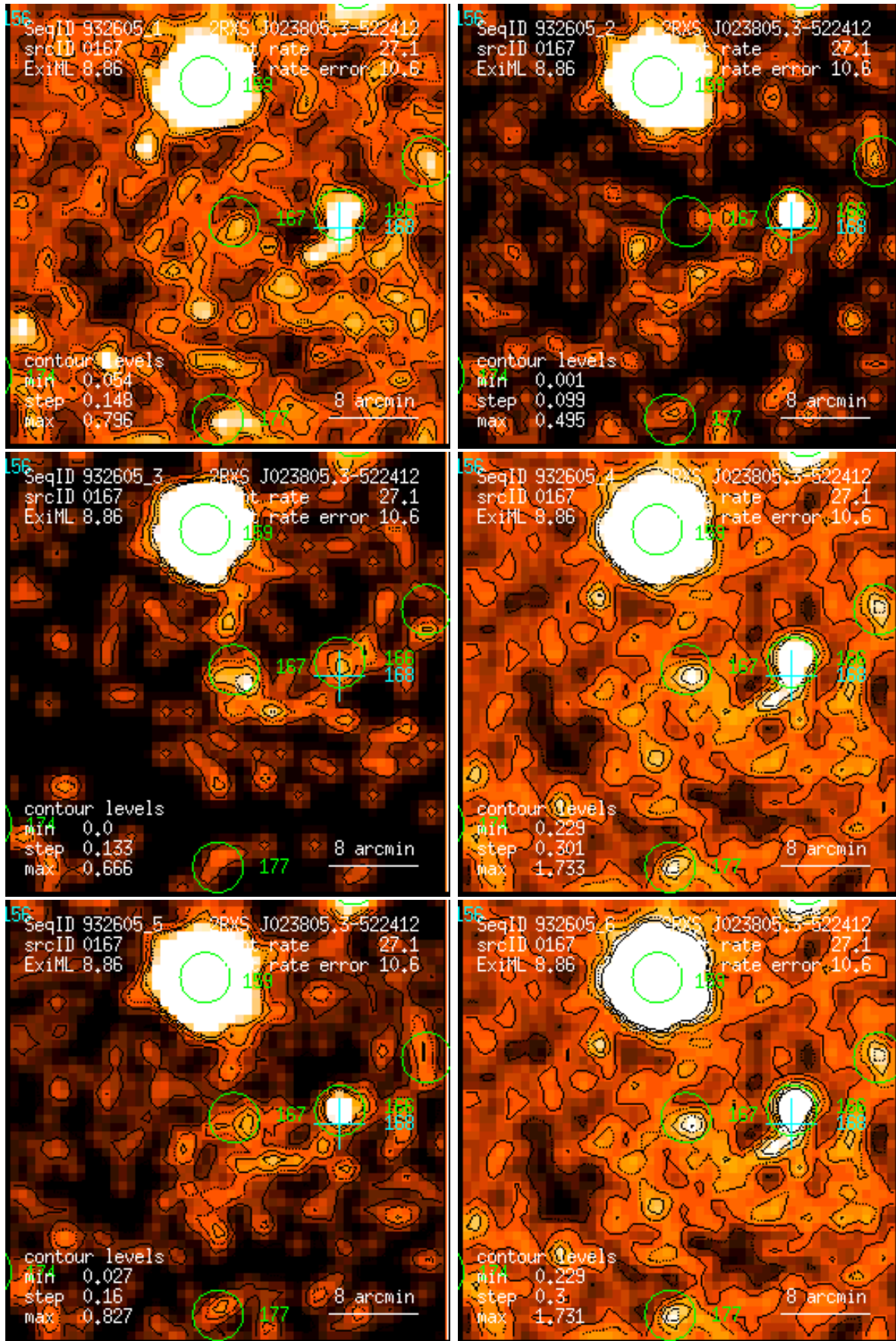
Figure 167: RASS 932605: detection 0167: band rate images, Gaussian filter: (1) PSPC channels 11 – 41, (2) 52 – 90, (3) 91 – 201, (4) 11 – 235, (5) 52 – 201, (6) 11 – 201. Broad band rates in counts/ks. Band rate contour levels in counts/ks/arcmin 2 .
