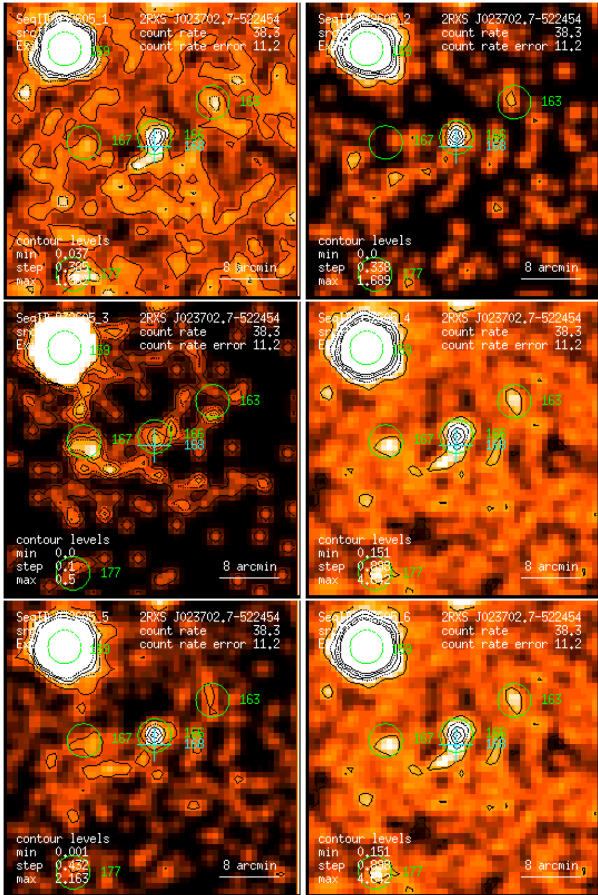
Figure 168: RASS 932605: detection 0168: band rate images, Gaussian filter: (1) PSPC channels 11 – 41, (2) 52 – 90, (3) 91 – 201, (4) 11 – 235, (5) 52 – 201, (6) 11 – 201. Broad band rates in counts/ks. Band rate contour levels in counts/ks/arcmin 2 .
