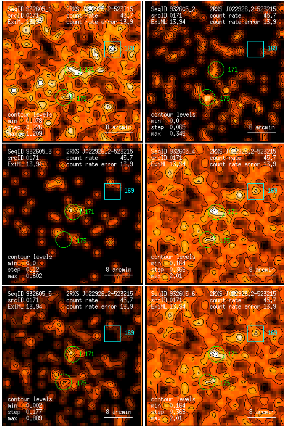
Figure 171: RASS 932605: detection 0171: band rate images, Gaussian filter: (1) PSPC channels 11 – 41, (2) 52 – 90, (3) 91 – 201, (4) 11 – 235, (5) 52 – 201, (6) 11 – 201. Broad band rates in counts/ks. Band rate contour levels in counts/ks/arcmin 2 .
