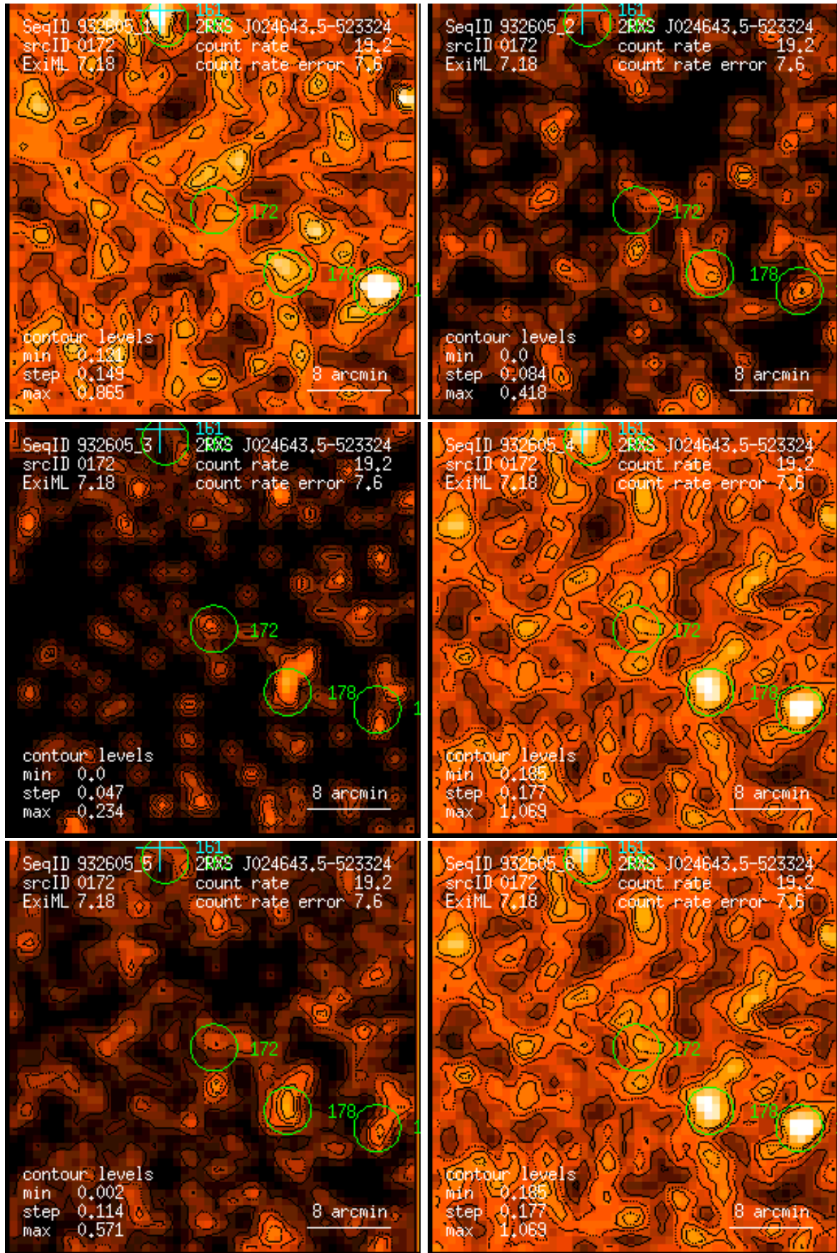
Figure 172: RASS 932605: detection 0172: band rate images, Gaussian filter: (1) PSPC channels 11 – 41, (2) 52 – 90, (3) 91 – 201, (4) 11 – 235, (5) 52 – 201, (6) 11 – 201. Broad band rates in counts/ks. Band rate contour levels in counts/ks/arcmin 2 .
