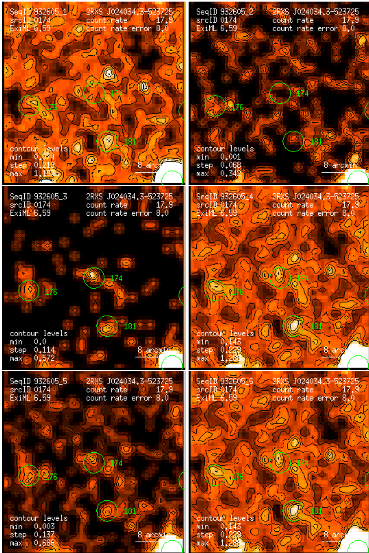
Figure 174: RASS 932605: detection 0174: band rate images, Gaussian filter: (1) PSPC channels 11 – 41, (2) 52 – 90, (3) 91 – 201, (4) 11 – 235, (5) 52 – 201, (6) 11 – 201. Broad band rates in counts/ks. Band rate contour levels in counts/ks/arcmin 2 .
