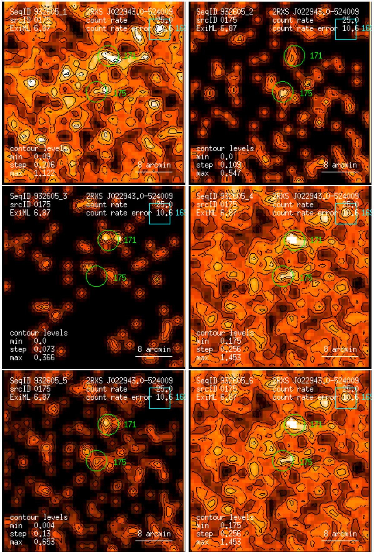
Figure 175: RASS 932605: detection 0175: band rate images, Gaussian filter: (1) PSPC channels 11 – 41, (2) 52 – 90, (3) 91 – 201, (4) 11 – 235, (5) 52 – 201, (6) 11 – 201. Broad band rates in counts/ks. Band rate contour levels in counts/ks/arcmin 2 .
