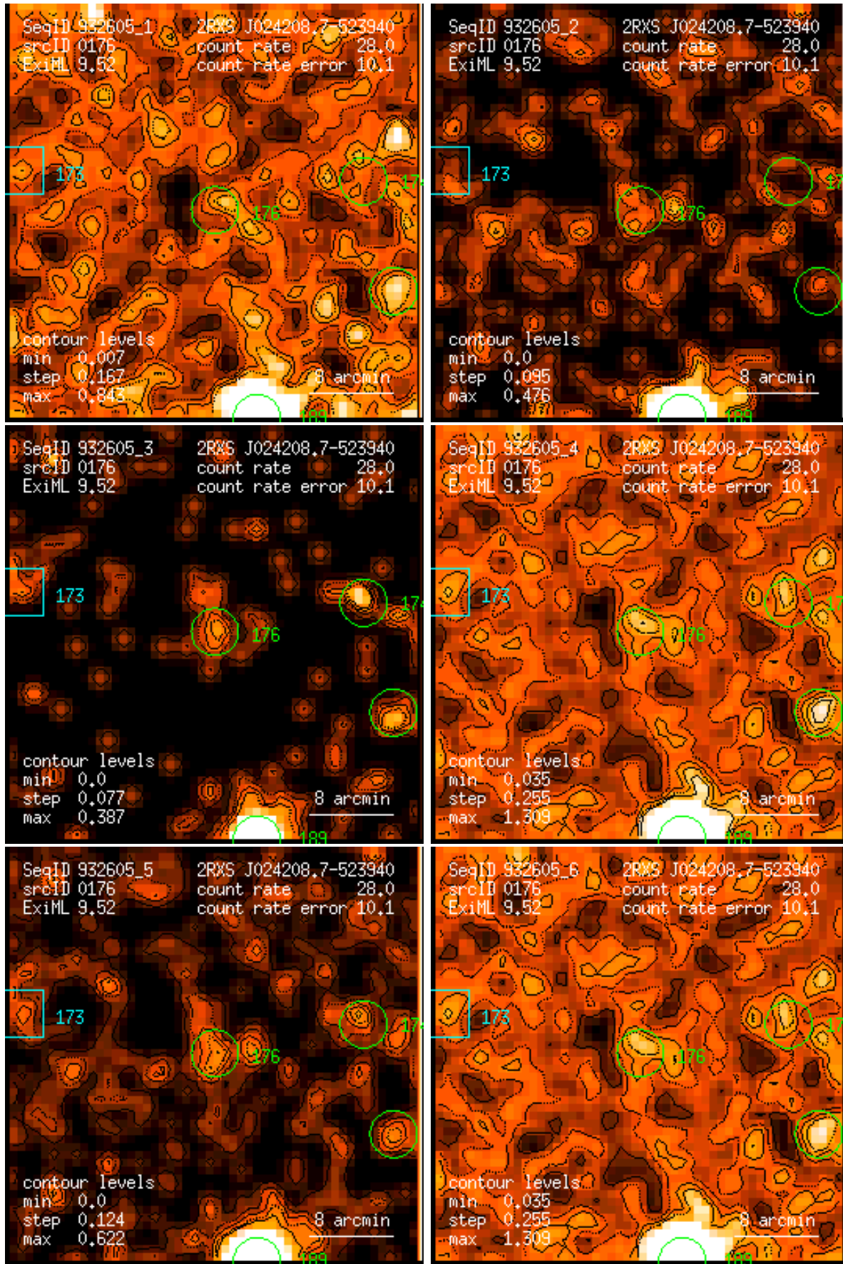
Figure 176: RASS 932605: detection 0176: band rate images, Gaussian filter: (1) PSPC channels 11 – 41, (2) 52 – 90, (3) 91 – 201, (4) 11 – 235, (5) 52 – 201, (6) 11 – 201. Broad band rates in counts/ks. Band rate contour levels in counts/ks/arcmin 2 .
